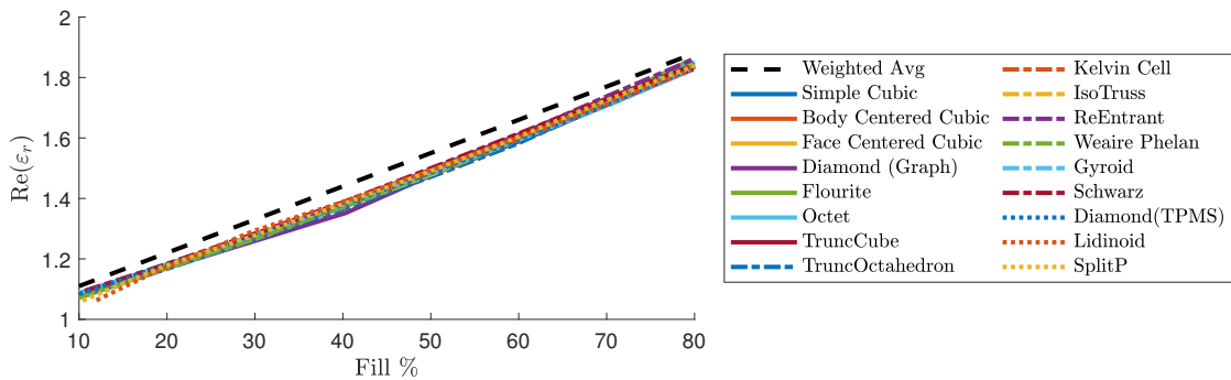
Fig. 3 — Results of lattice simulation study, compared to weighted average approximation.
