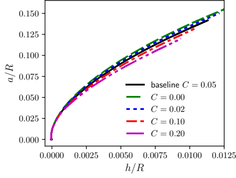
(a) contact radius vs. depth
