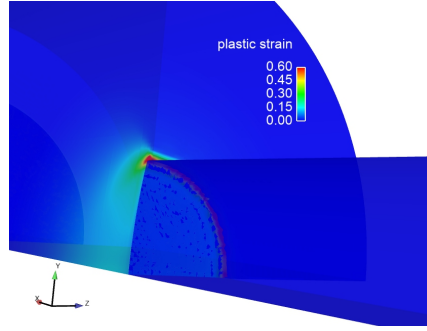
(a) plastic strain, 5\times vel
