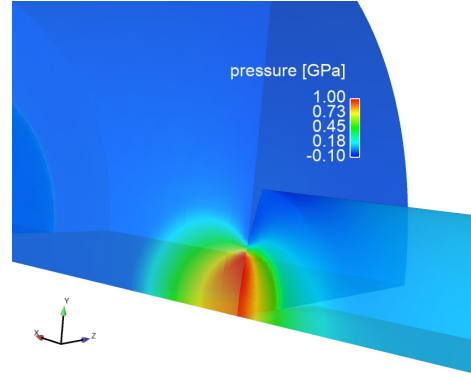
(b) local pressure
