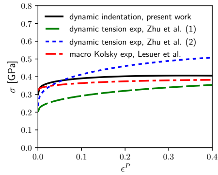
(b) uniaxial stress-strain, 1/s
