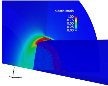
(c) plastic strain, 10\times vel
