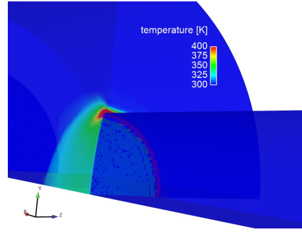
(b) temperature, 5\times vel
