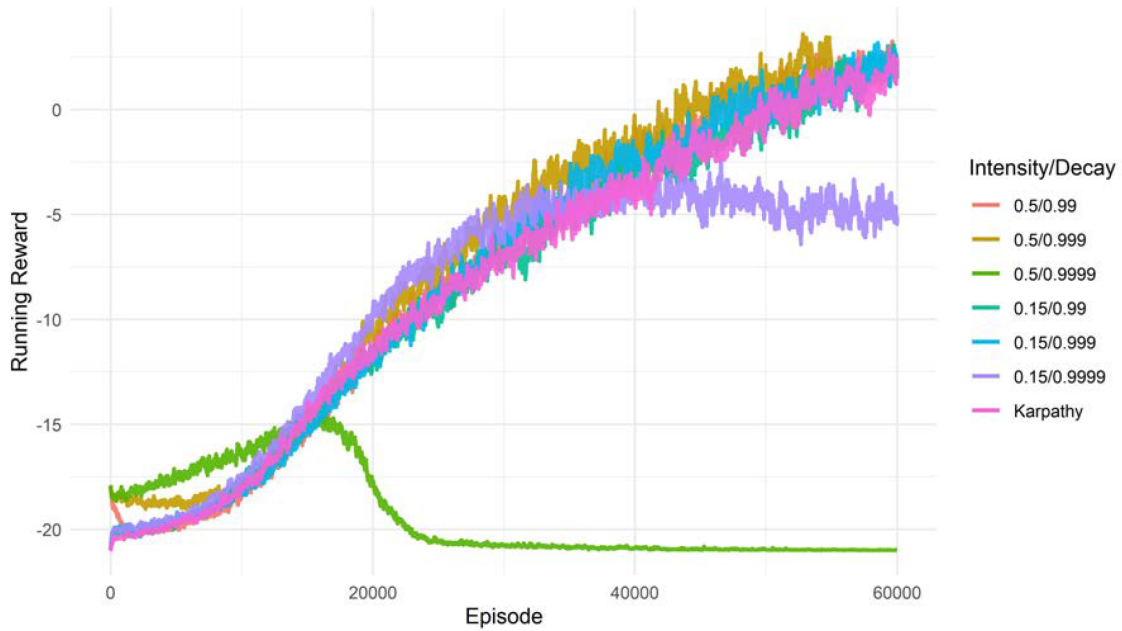
Figure 2.4: Agents trained with near-zero intensity or moderately low intensity and high decay levels did not collapse, but in effect were more akin to regular agents than being assisted by human logic. Source: [3]
