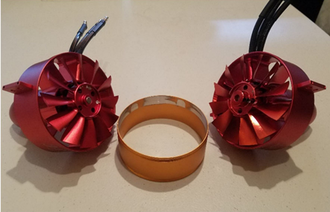
Figure 6. CREDF system before assembly.
