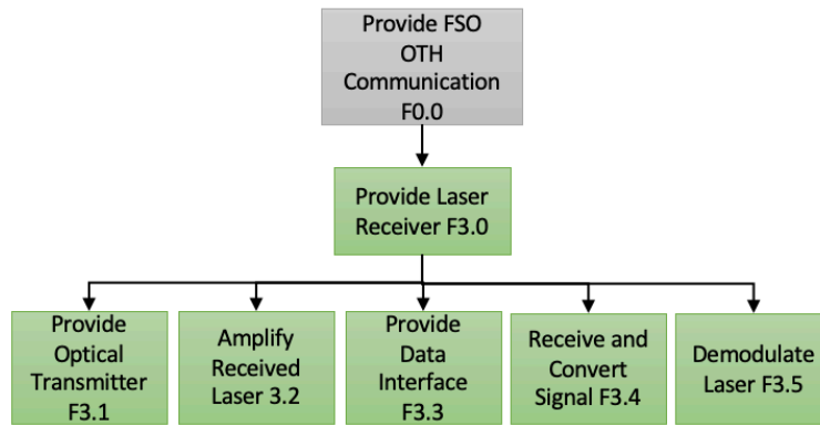
Figure 13. Laser Receiver Functional Model
