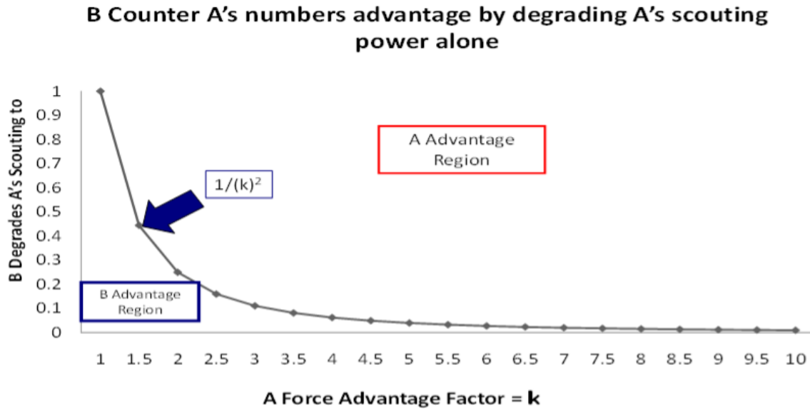
Figure 9. Relationship between scouting and force advantage based on Salvo Equations 284
