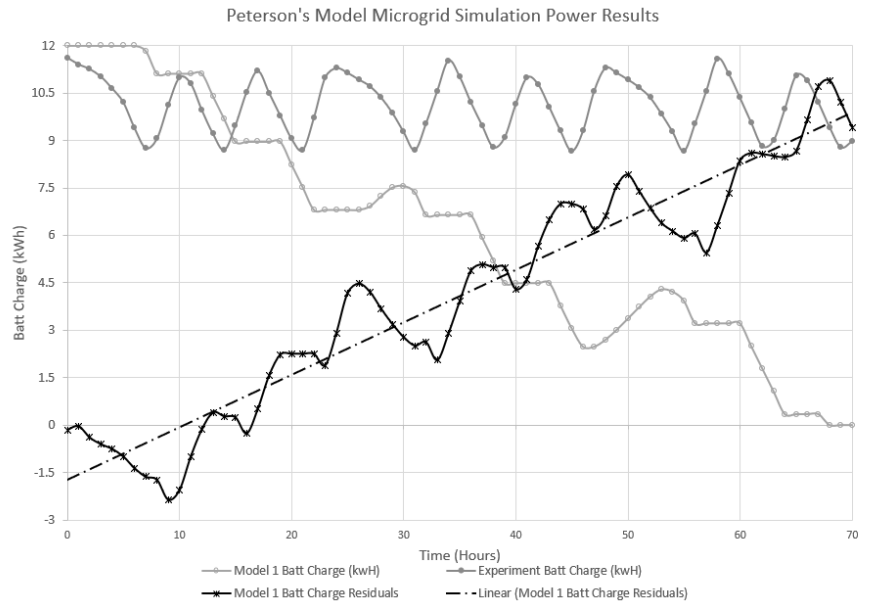
Figure 1. Peterson's Simulation Model battery charge results show a positive trend because the model batteries were not charged by excess diesel generator power.
