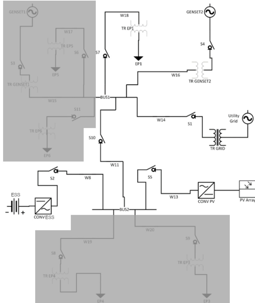
Figure 2.5. Peterson's Simulation model adjusted architecture with excess components removed in grey to match scaled experiment generators and loads. Adapted from [57].
