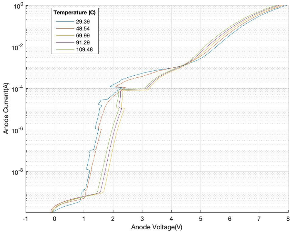
Figure 41. Device C2 Forward Bias Curves Post Initial Stress Test
