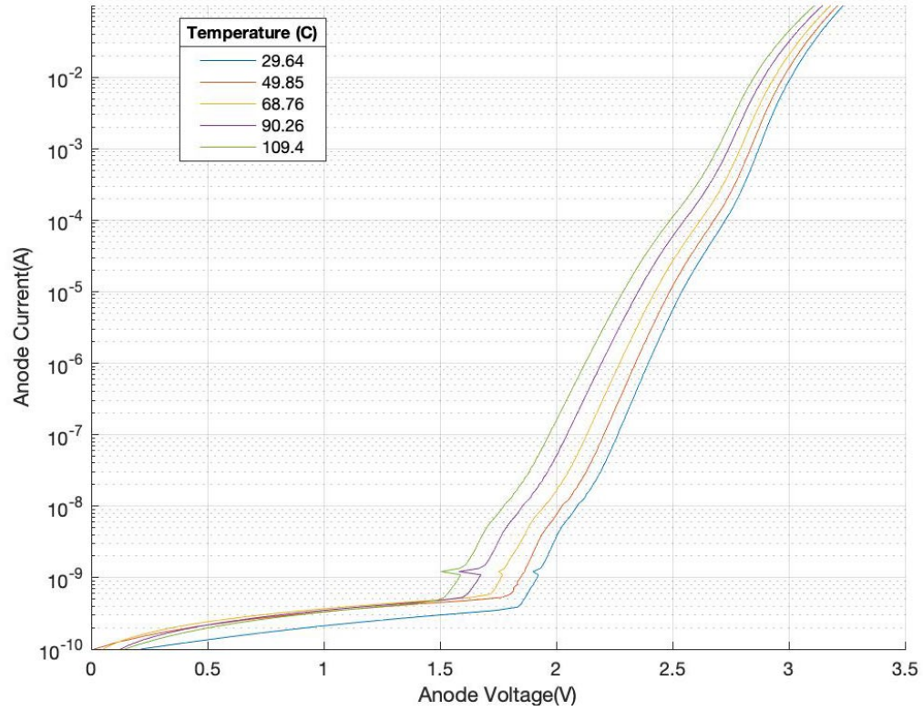
Figure 13. Initial Forward Bias Curves for N1 Device
