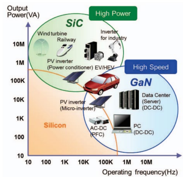
Figure 1. Applications of WBG Semiconductors GaN and SiC in Relation to Silicon. Source: [6].
