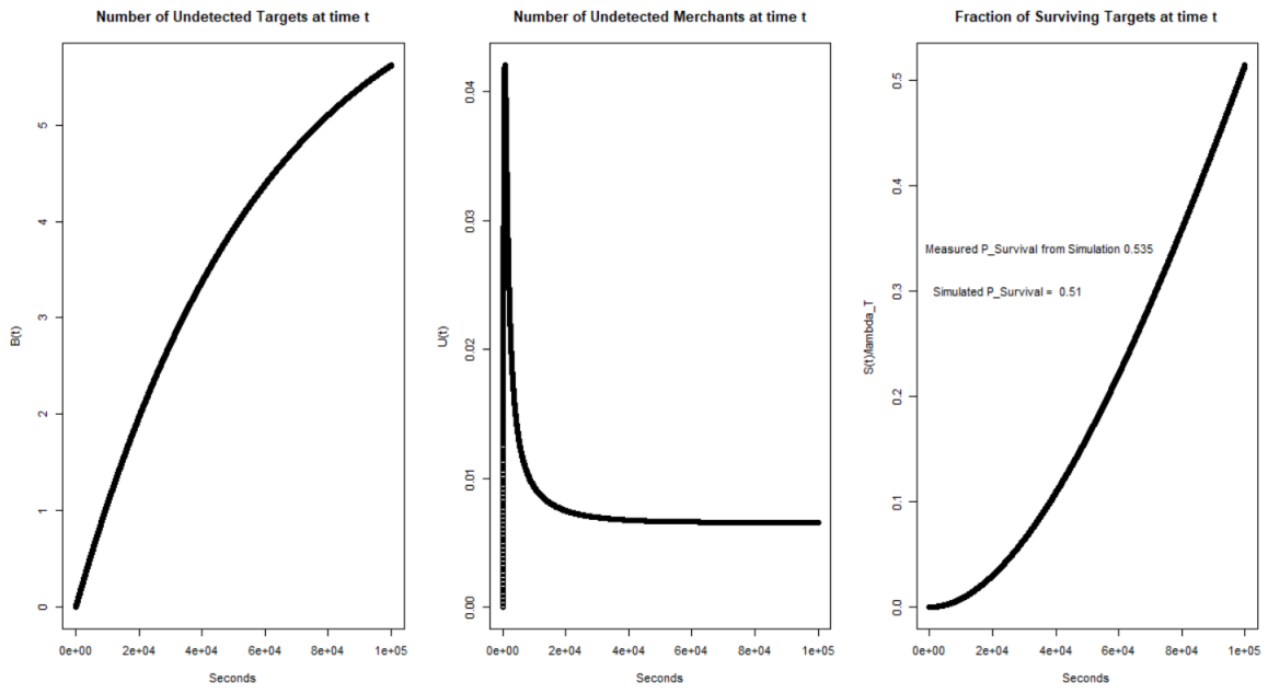
Figure 3.3. Plots of B(t) , U(t) , and \frac{Z(t)}{\lambda_T t}
