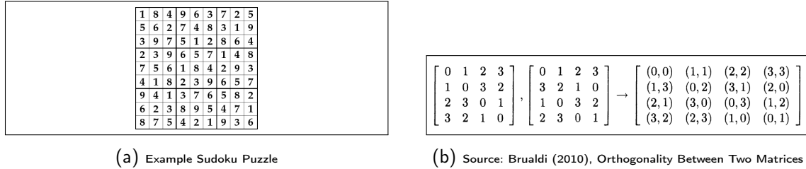
Figure A.1. Latin Squares
