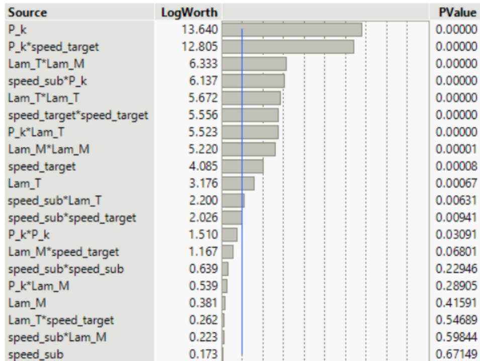
Figure 4.28. Regression Including Full Factorial Effects to Degree 2, Surface Action Group, No Communication
