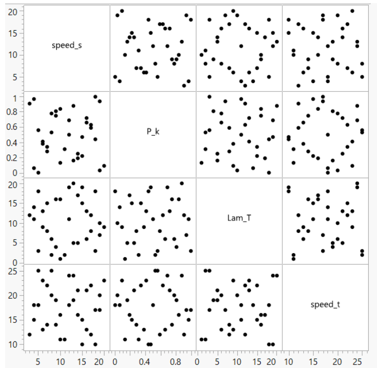
Figure A.2. Geometry of NOLH Visible When Viewed as a Scatterplot Matrix Between Several Factors
