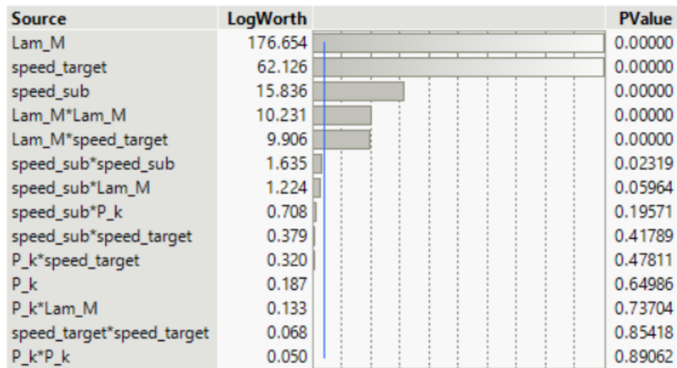
Figure 4.33. Regression Including Full Factorial Effects to Degree 2, Surface Action Group, Intermittent Communication
