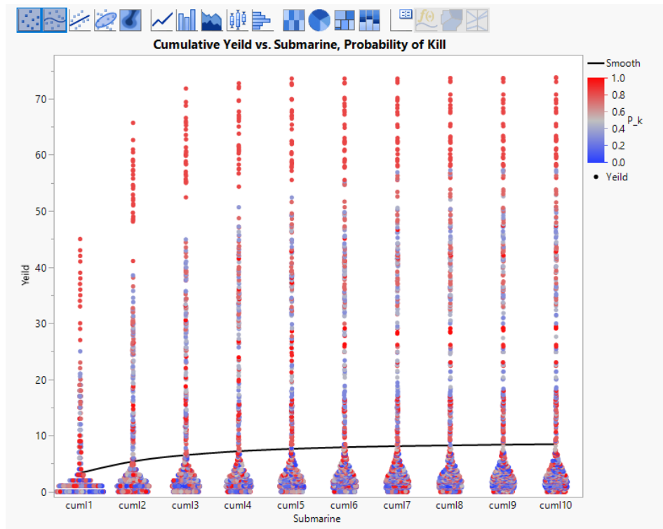
Figure 4.14. Cumulative Yield by Submarine, P_K , Interfering Contacts, Intermittent Communication
