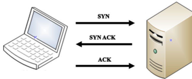
Figure 2.3. TCP "3-way-handshake"
