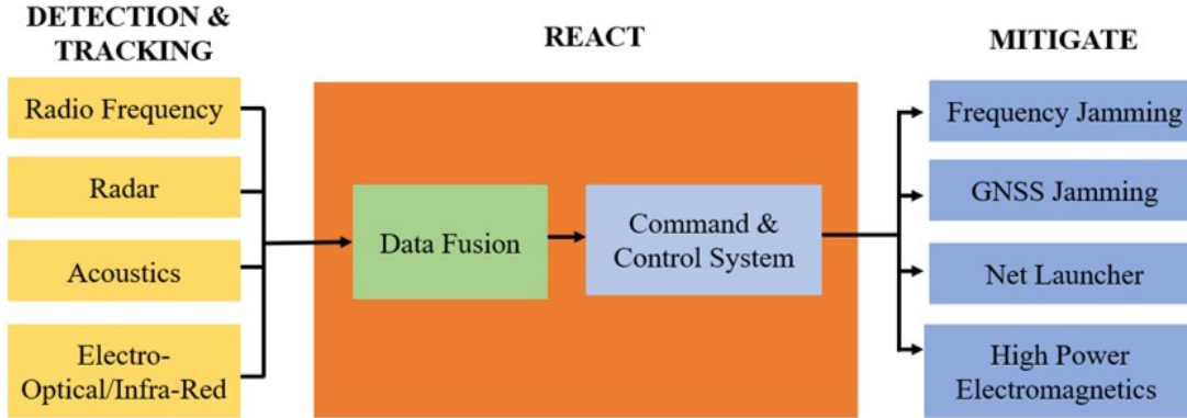
Figure 2.2. C-UAS Network [44]
