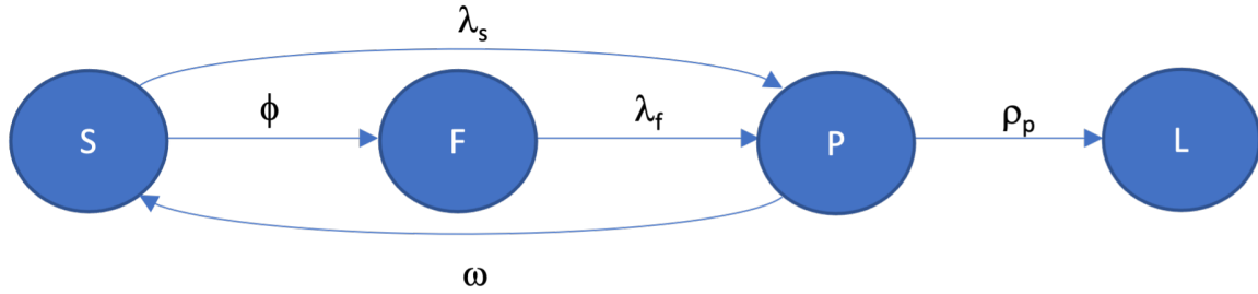
Figure 2.2. Reduced Markov Model of Condenser Tube Failures.
