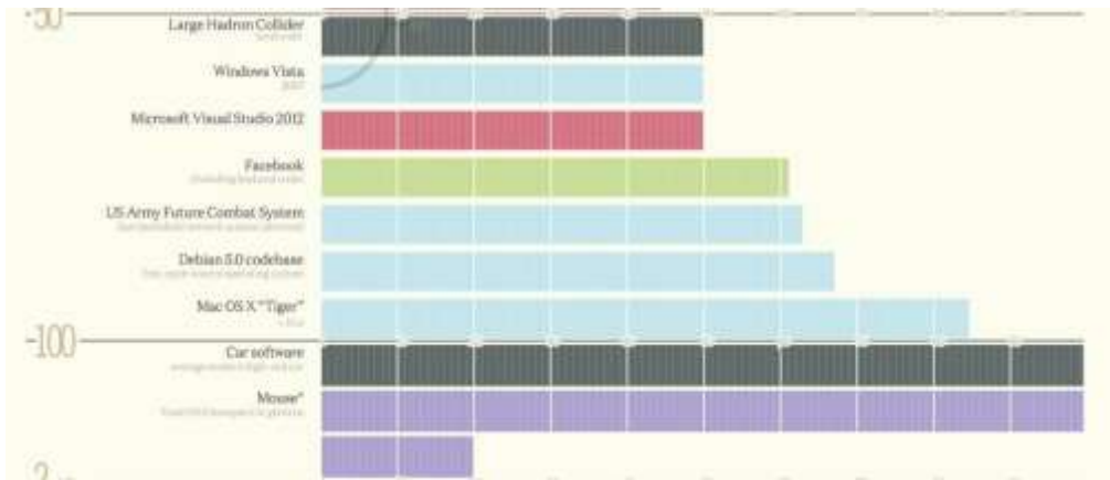
Source: https://informationisbeautiful.net/visualizations/million-lines-of-code/
