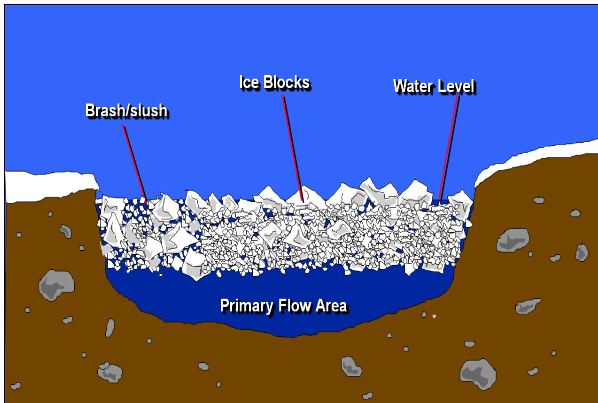
Figure 10. Diagram of break-up jam cross section.
