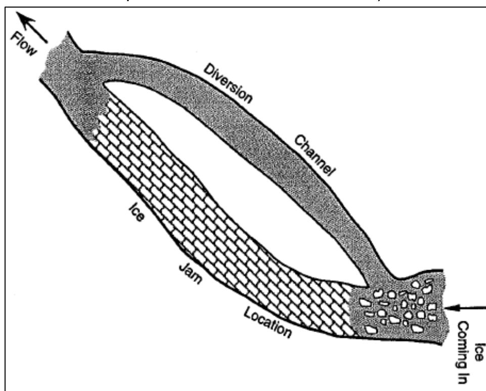
Figure 37. Diversion channel schematic for ice jam flood control. (Image reproduced from USACE 2002. Public domain.)
