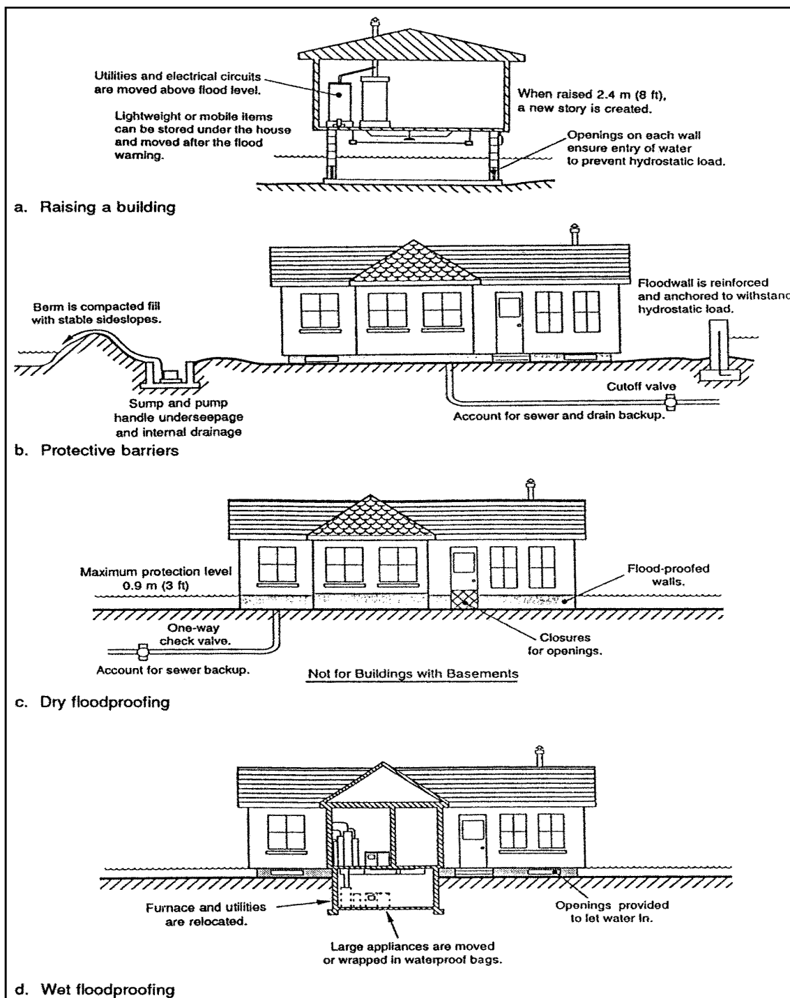
Figure 39. Floodproofing techniques. (Image reproduced from USACE 2002. Public domain.)
