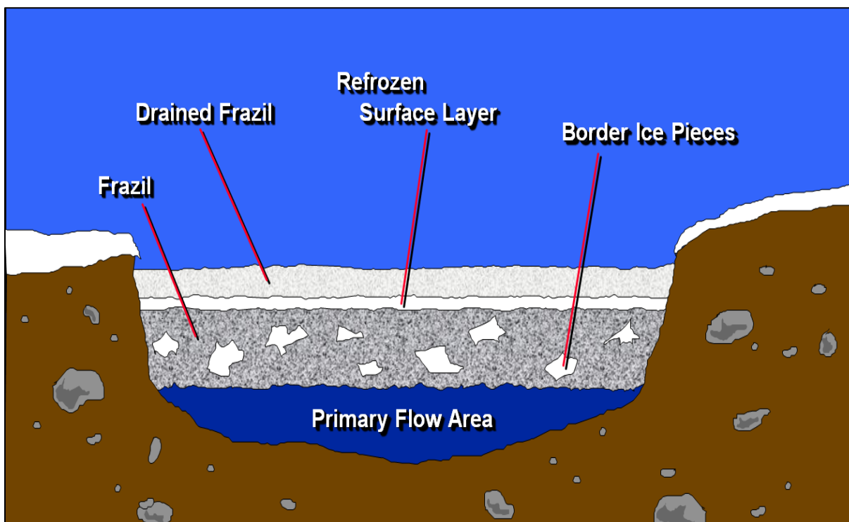
Figure 7. Diagram of freeze-up jam cross section.
