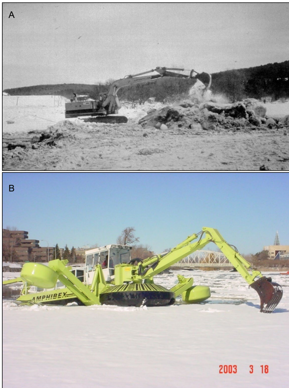
Figure 27. Excavator used to remove ice jam (A) (image reproduced from USACE 2002) and Amphibex specialized equipment (B). (Image reproduced with permission from Normrock Industries Inc.)
