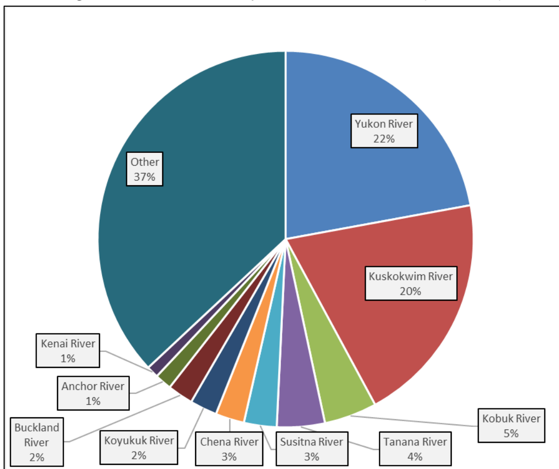
Figure 15. Ice Jam distribution by river based on IJDB records (1889–2022).
