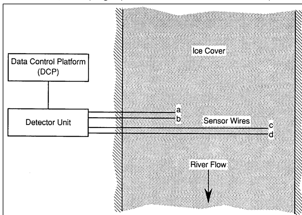
Figure 26. CRREL ice jam motion detector using a trip wire; installed on the Kennebec River, Maine. (Image reproduced from Zufelt 1993. Public domain.)
