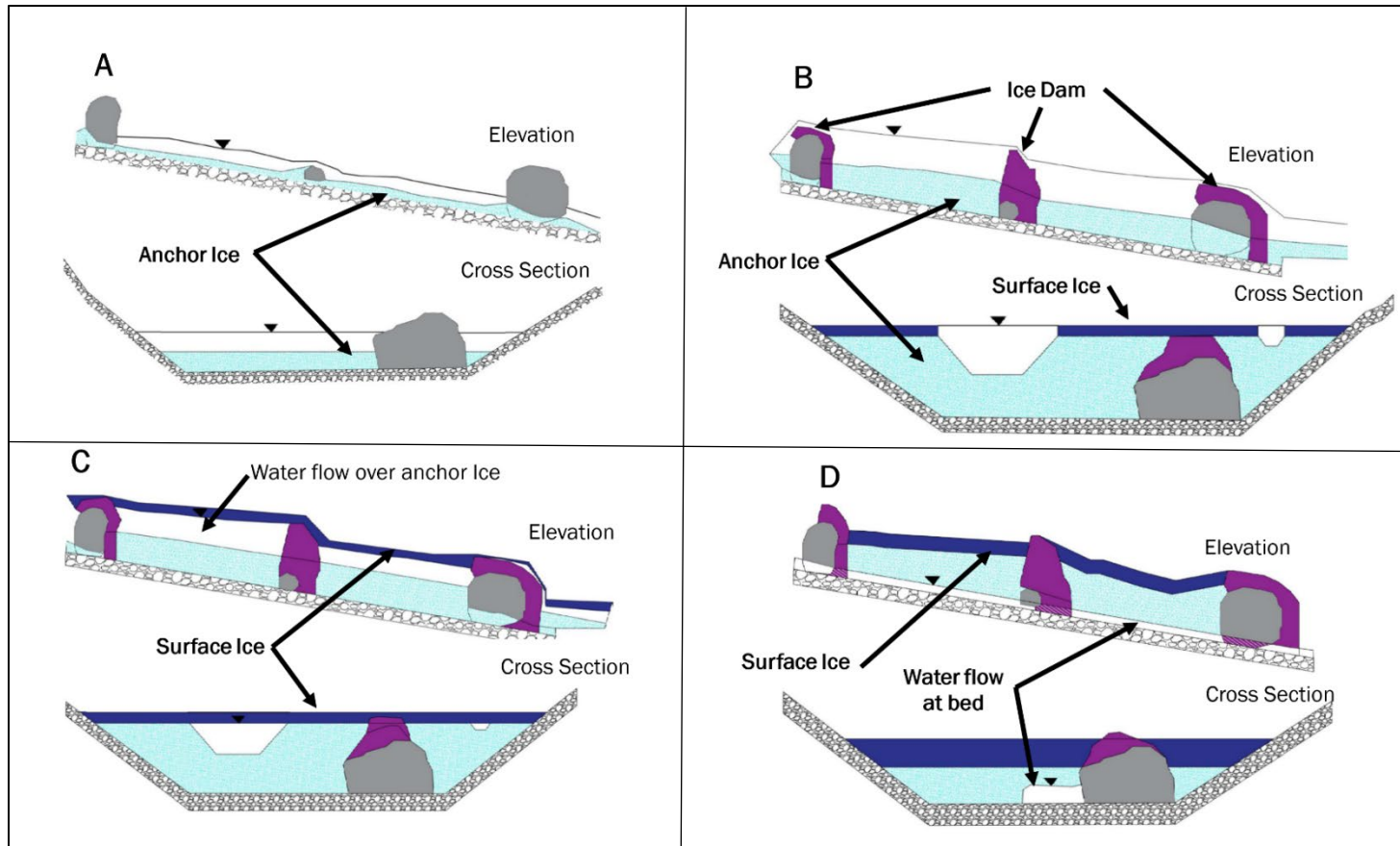
Figure 9. Anchor ice dam progression concept. (Image reproduced from Daly et al. 2019. Public domain.) Early-stage anchor ice formation along stream bed ( A ). Ice dam formation around large cobbles or boulders with subsequent rise in water level and some surface ice development ( B ). Full ice-cover formation across the channel ( C ). Ice dam breaching and anchor ice detachment. Note flow along stream bed at this stage ( D ).
