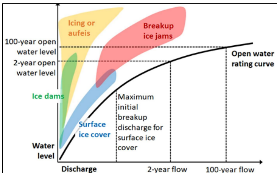
Figure 40. Concept of ice processes influence on water level above an open water rating curve. (Image reproduced with permission from Burrell et al. 2021.)
