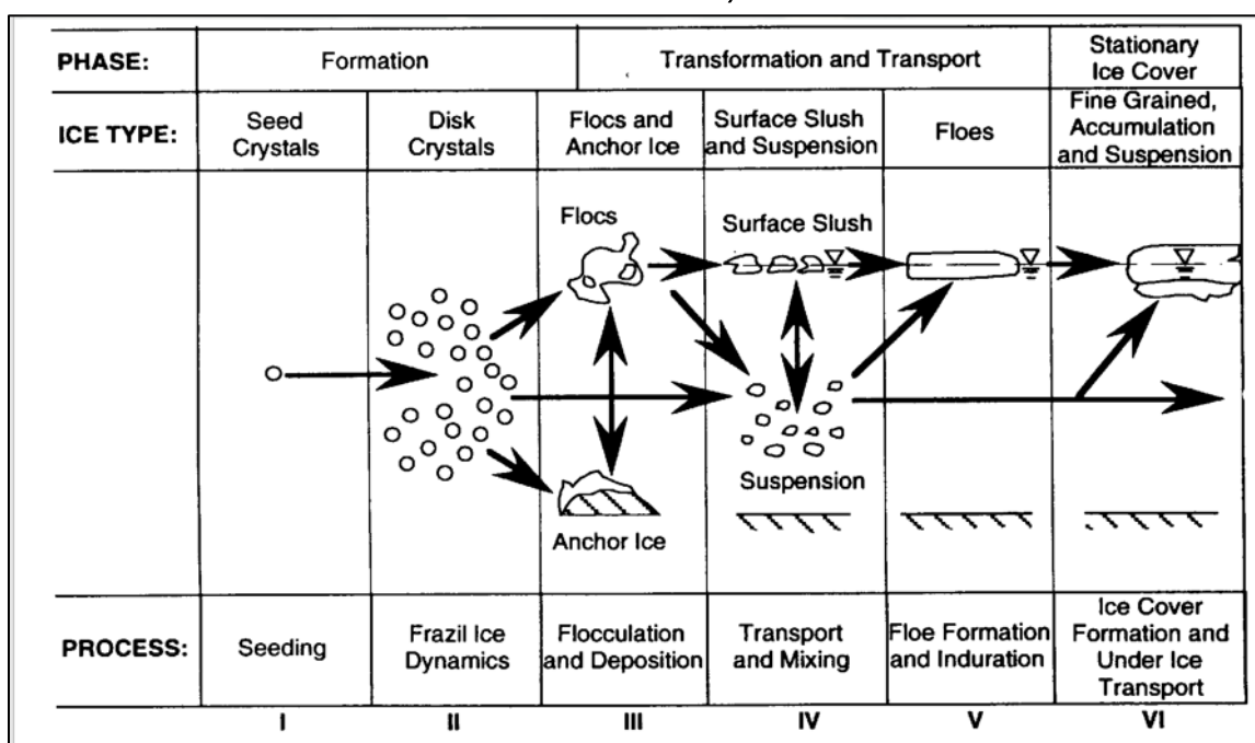
Figure 1. Evolution of frazil ice in natural water bodies. (Image reproduced from Daly 1994. Public domain.)
