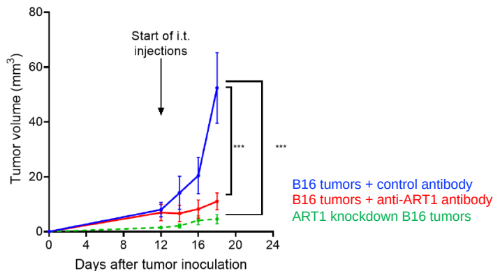
Figure 1. Effect of anti-ART1 antibody on B16 melanoma cell tumorigenesis. See text for details.
