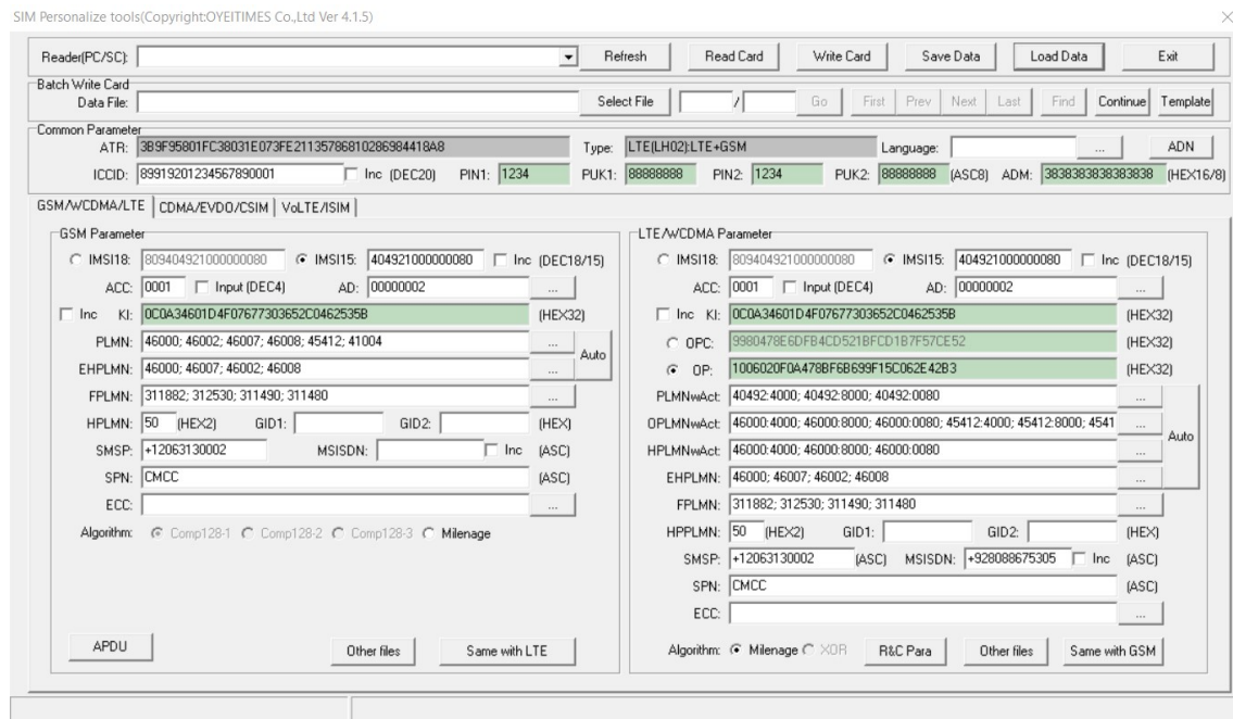
Figure 3.9. OYSIMWrite SIM Card User Interface. Source: [32].
