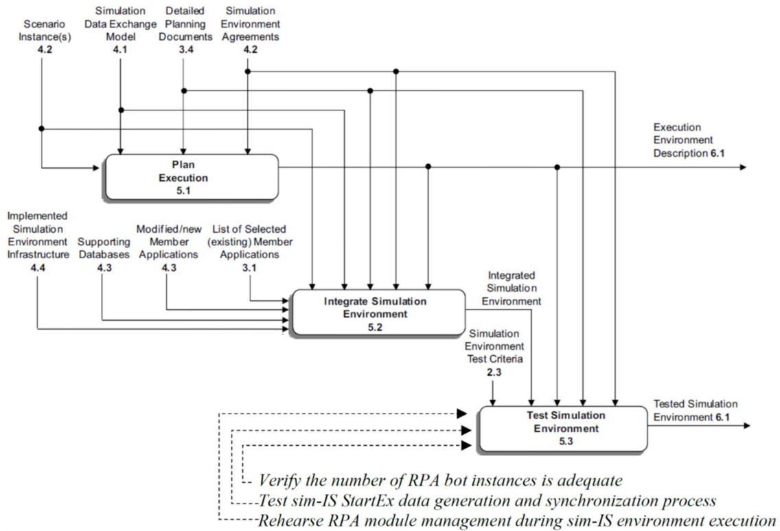
Figure 62. DSEEP Step 5: Integrate and Test Simulation Environment.
