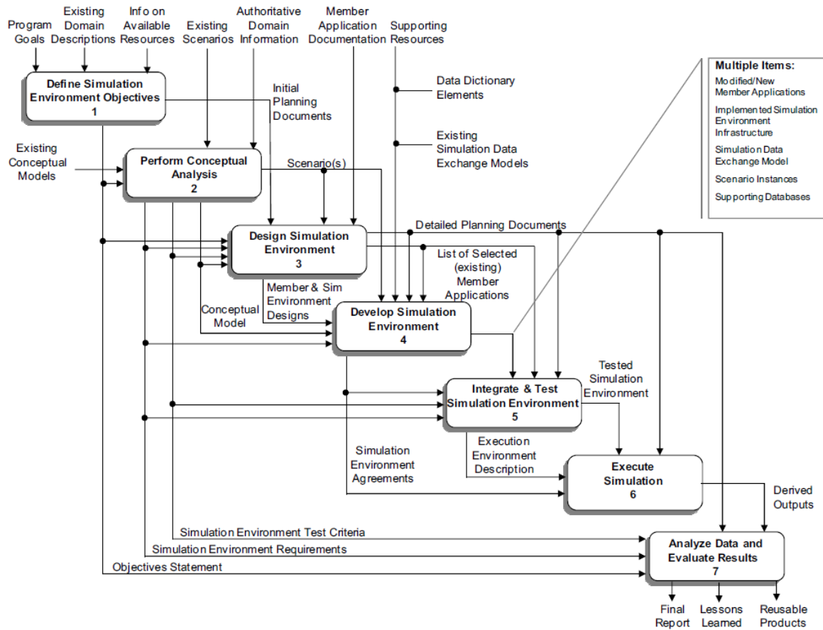
Figure 56. Detailed DSEEP View. Source: IEEE Std 1730 (2011) © 2011 IEEE.
