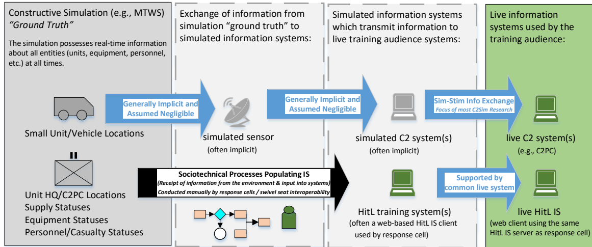
Figure 3. The Layers of Sim-IS Interoperability.
