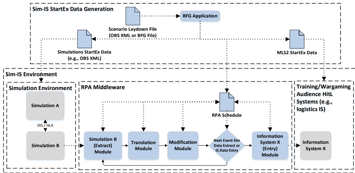
Figure 30. Sim-IS RPA Architecture.
