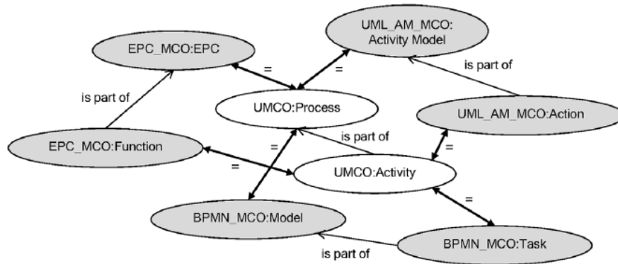
Figure 18. Extract of the UMC0 Showing Semantic Alignment of Modeling Languages. Source: Fengel (2013).
