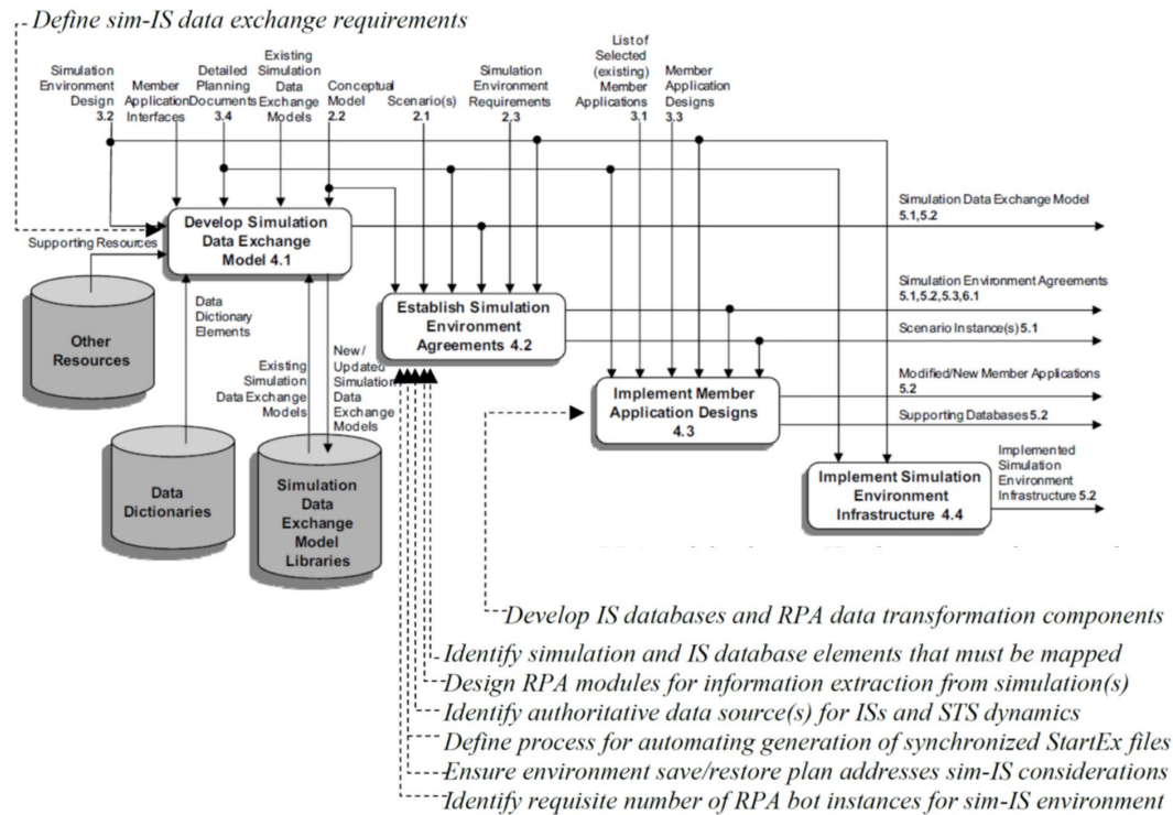
Figure 61. DSEEP Step 4: Develop Simulation Environment. Source: IEEE Std 1730 (2011) © 2011 IEEE.
