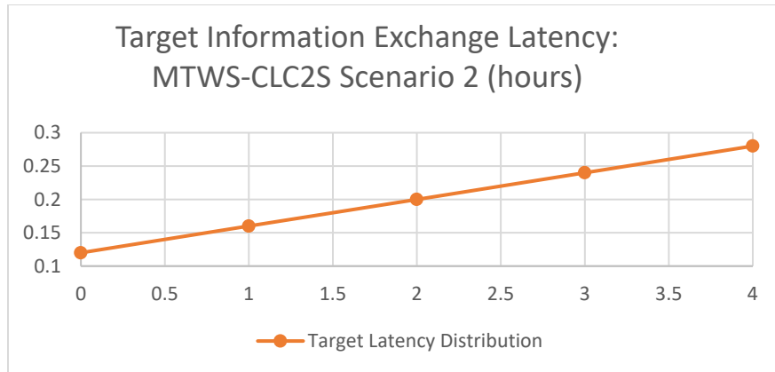
Figure 45. Target Latency Distribution for MTWS-CLC2S Simulation 2 (Linear Distributions).
