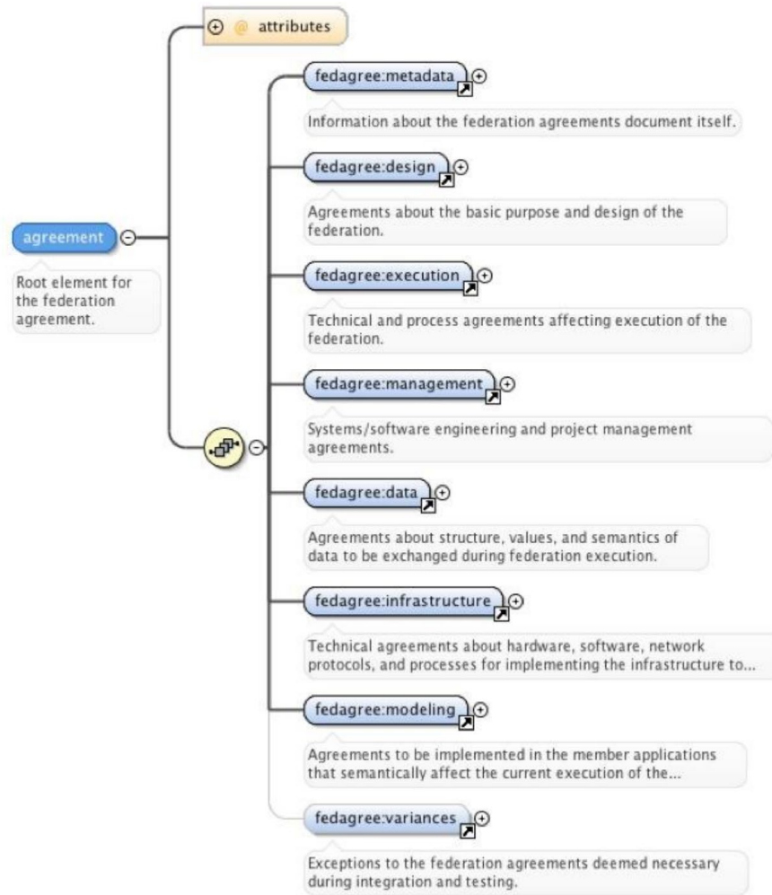
Figure 65. Top-level View of the FEAT Schema. Source: SISO FEAT Product Support Group (2017).
