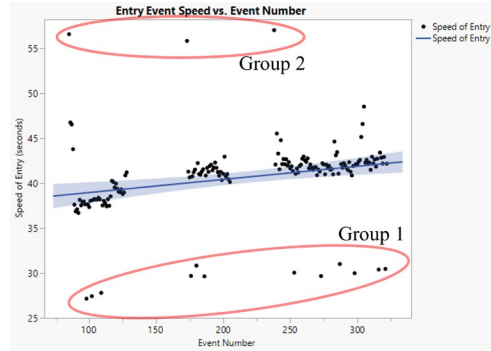
Figure 51. Speed of MTWS-CLC2S RPA Entry Events (in Seconds) Relative to Their Time of Execution.
