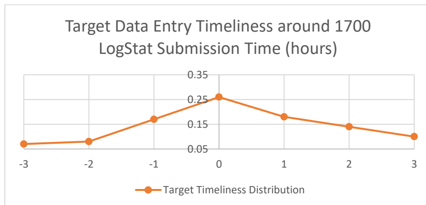
Figure 44. Target Timeliness Distribution for JCATS-CLC2S Simulation and MTWS-CLC2S Simulation 1 (Unimodal).
