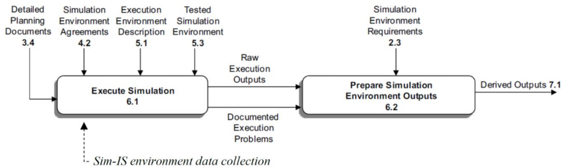
Figure 63. DSEEP Step 6: Execute Simulation. Source: IEEE Std 1730 (2011) © 2011 IEEE.
