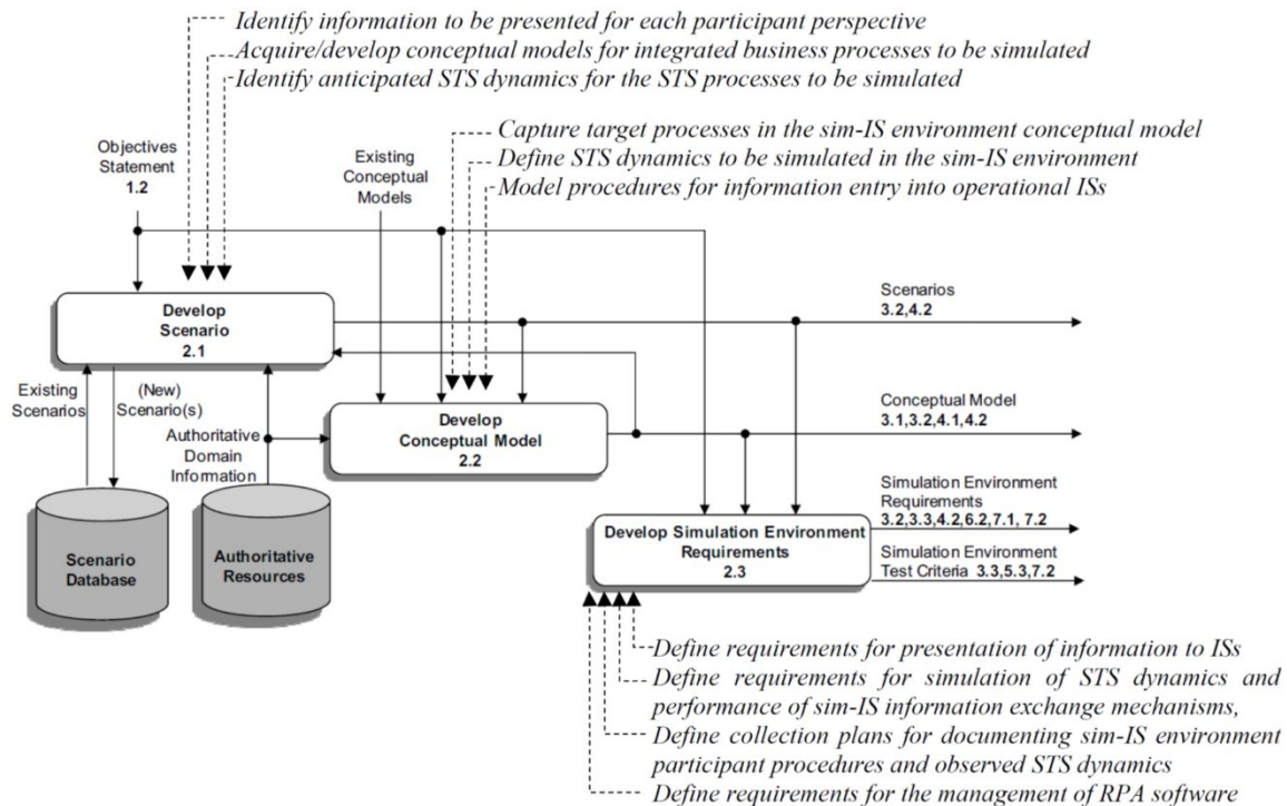
Figure 58. DSEEP Step 2: Perform Conceptual Analysis. Source: IEEE Std 1730 (2011) © 2011 IEEE.
