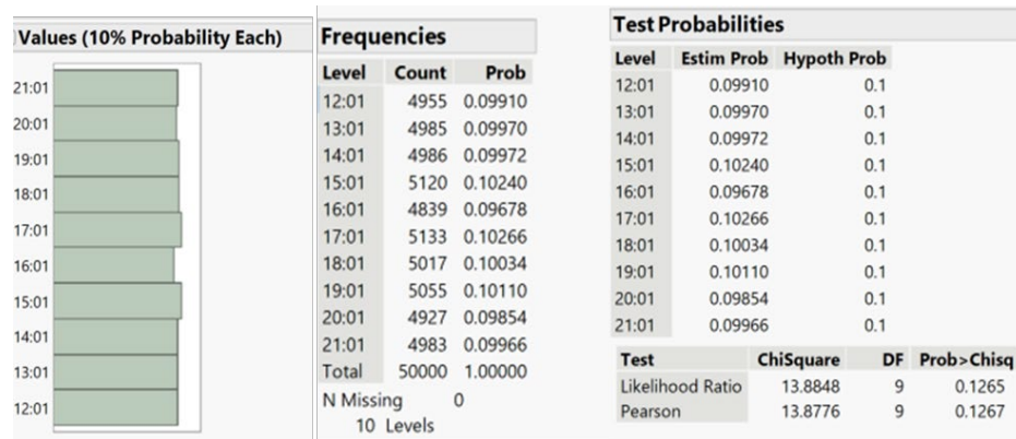
Figure 77. Results of UiPath PRNG Randomness Testing
