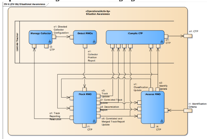
Figure 1. Example of a structured modeling notation (UML). From “Simulation environment architecture development using the DoDAF,” by van den Berg, T.V. and Lutz, R., 2015, Fall SISO Simulation Interoperability Workshop, p. 7.
