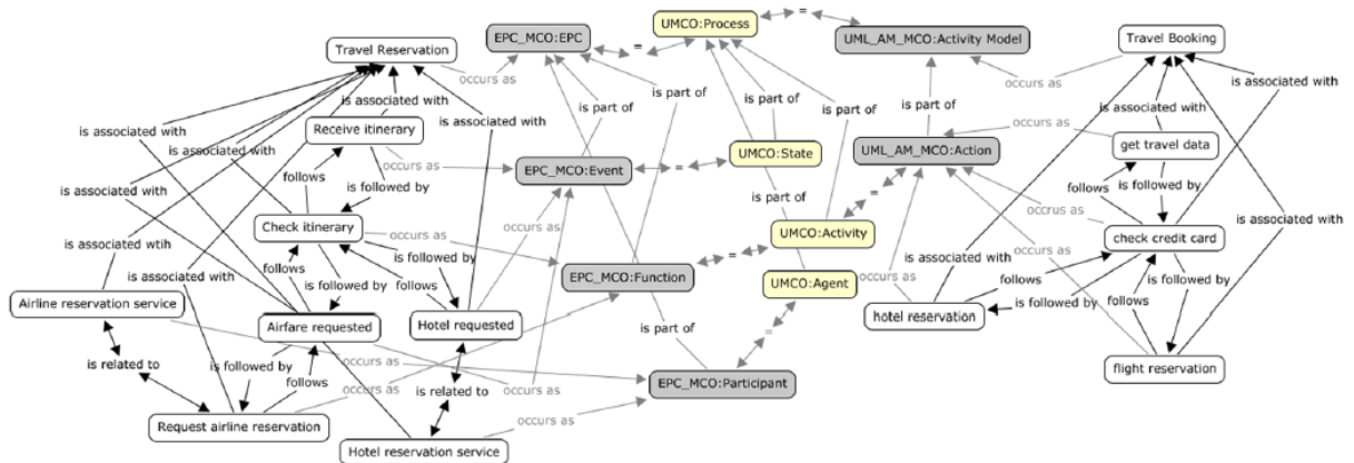
Figure 19. Aligning Event-Driven Process Chain (EPC) and UML Modeling Language Semantics via UMC0. Source: Fengel (2013).
