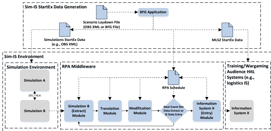
Figure 1. RPA-based sim-IS information exchange architecture
