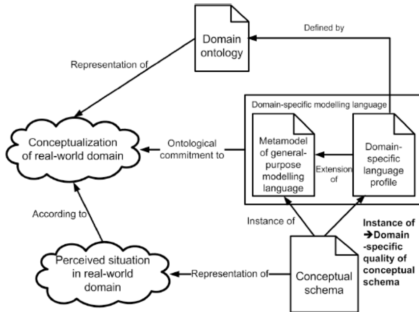
Figure 13. Domain Ontology-based Conceptual Modeling Approach. Source: Gailly and Poels (2010).
