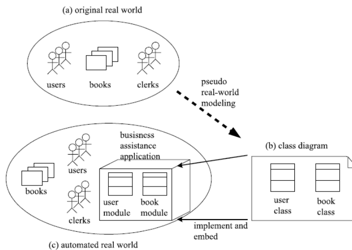
Figure 17. Pseudo Real-World Modeling: Usage 3. Source: Isoda (2001).
