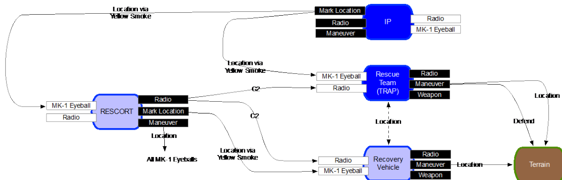
Figure 3. Example of Entity Subset Conceptual Model of a MVCM model. From Morse K.L. and Drake D.L. (2020), p. 15.
