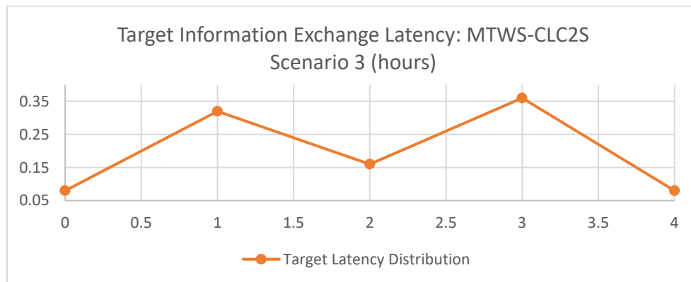
Figure 47. Target Latency Distribution for MTWS-CLC2S Simulation 3 (Bimodal Distributions).
