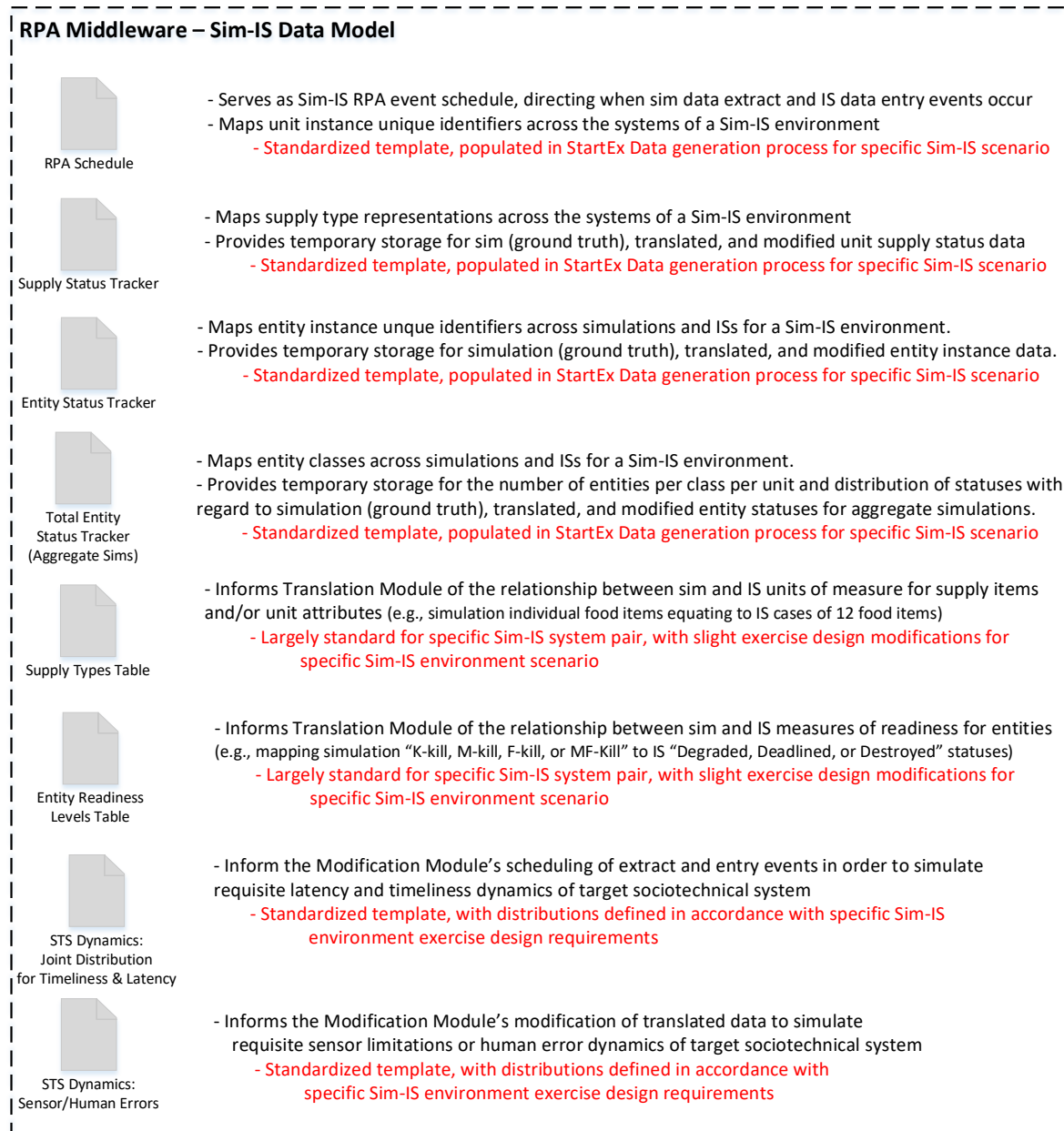
Figure 32. Sim-IS Data Transformation Components.
