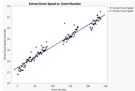
Figure 50. Speed of MTWS-CLC2S RPA Extract Events (in Seconds) Relative to Their Time of Execution.
