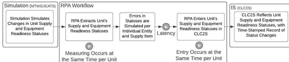
Figure 42. Conceptual Model of Sim-IS Environment for Simulation of LogStat Submission Process.
