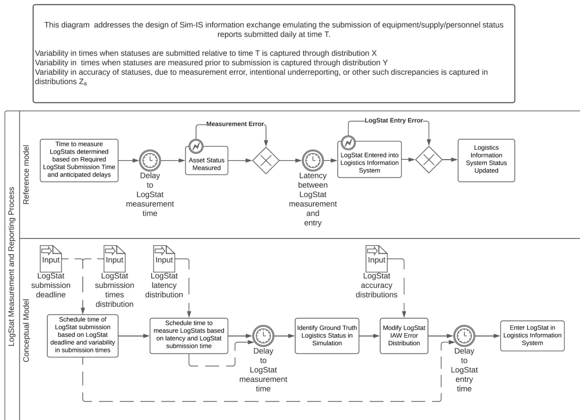
Figure 35. Conceptual Model of Sociotechnical System Dynamics Simulated in a Sim-IS Environment.
