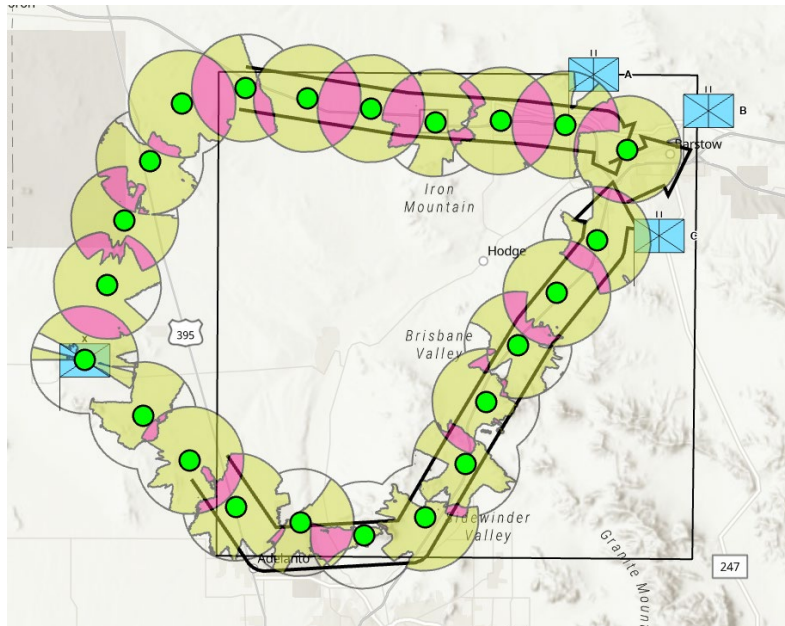
Figure 20. Communication Coverage for Network Operating on 2.4 GHz, with Aerostat Deployed at 300 ft
