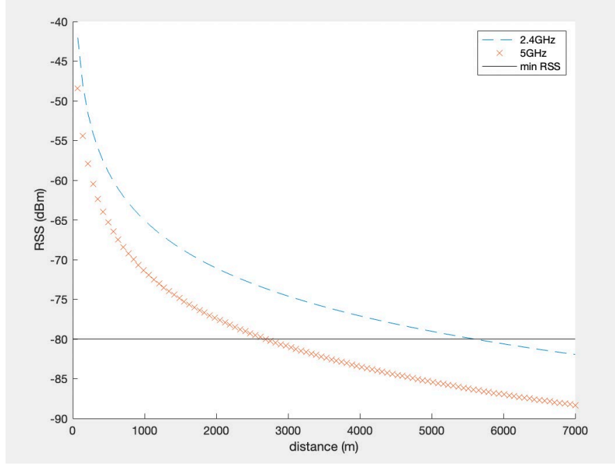
Figure 11. Received Signal Strength as a Function of Distance when Operating at 2.4 GHz and 5GHz.
