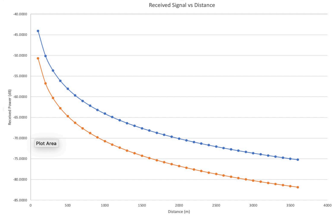
Figure 13. Comparing 2.4 GHz and 5GHz Received Signal Strength to Distance
