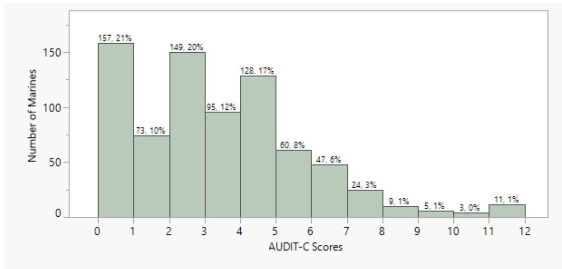
Figure 22. AUDIT-C Scores
