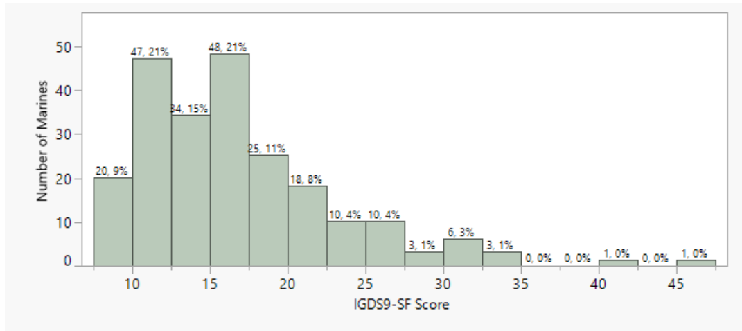
Figure 36. IGDS9-SF Scores
