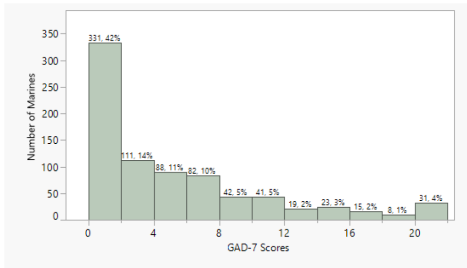
Figure 17. GAD-7 Scores
