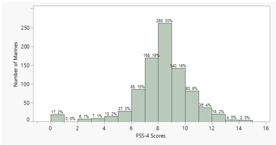
Figure 12. PSS-4 Scores.
