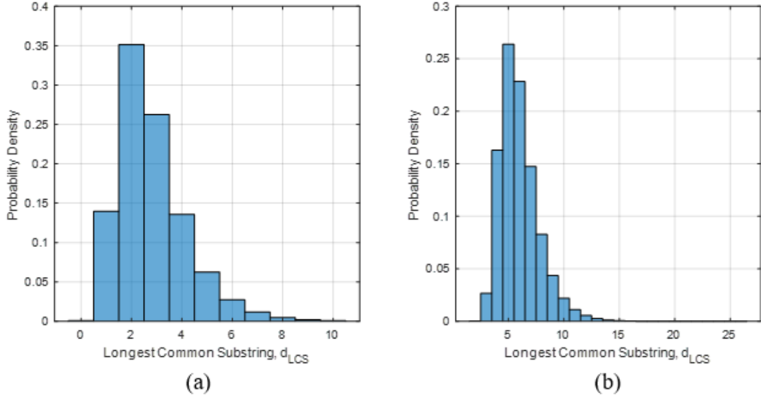
Figure 13. Histogram of Normalized LCS Results Between One Sequence and 2^{15} Randomly Generated Sequences of Length (a) \varepsilon = 10 and (b) \varepsilon = 100
