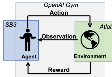
Figure 10. Relationship Between Atlatl, OpenAI Gym, and SB3
