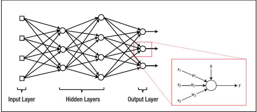
Figure 8. Deep Neural Network. Source: [1].
