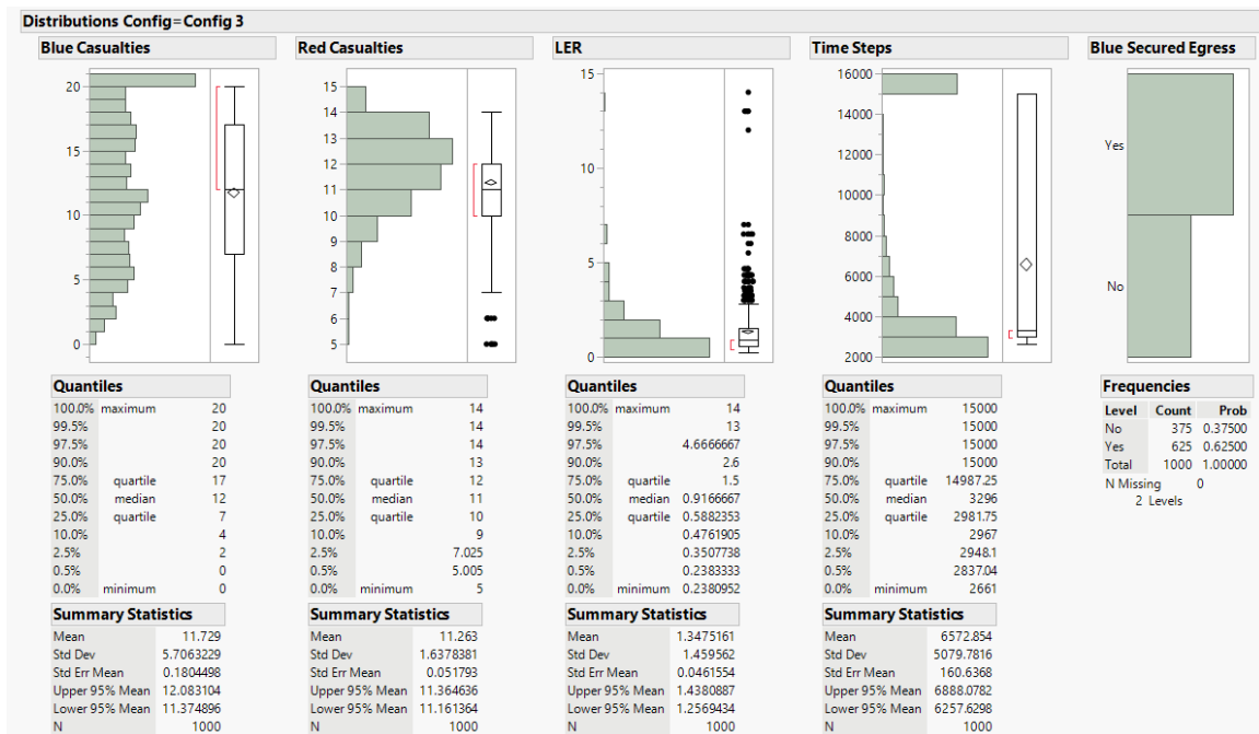
Figure 24. Statistical Summary of Baseline Simulation Experiment Configuration (Configuration 3)
