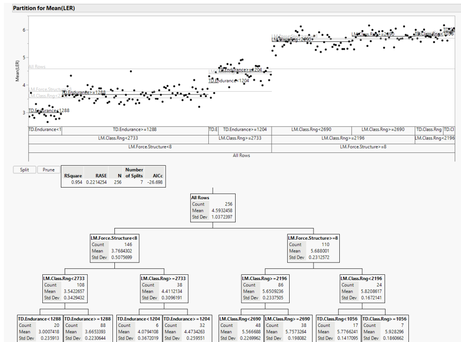
Figure 33. Partition Tree for LER
