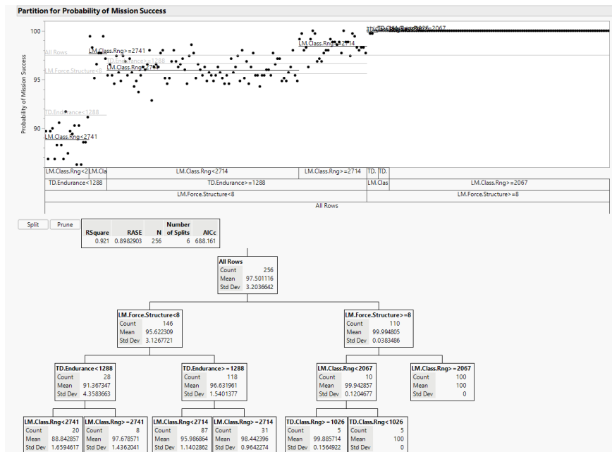
Figure 35. Partition Tree for Probability of Mission Success
