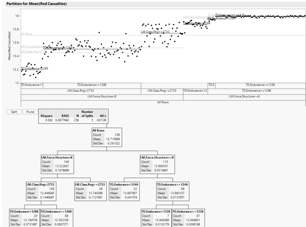
Figure 32. Partition Tree for Red Force's Casualties
