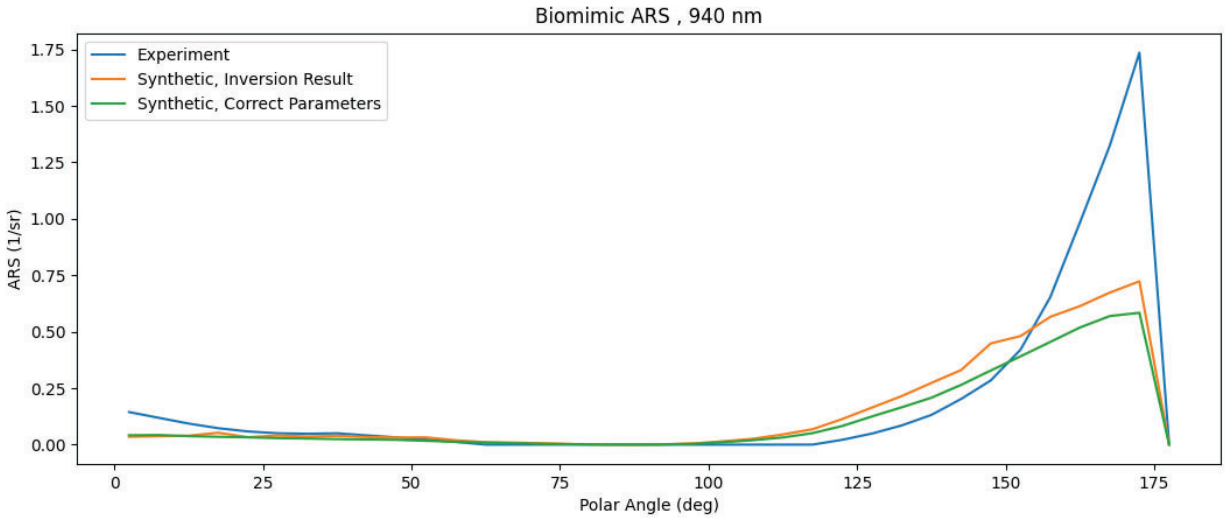
Figure 13. Experimental and synthetic Biomimic ARS datasets
