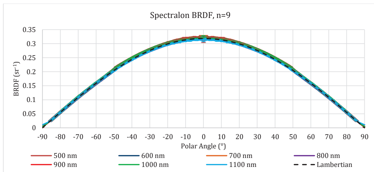
Figure 16. Multispectral BRDF measurements of the Spectralon reflectance standard
