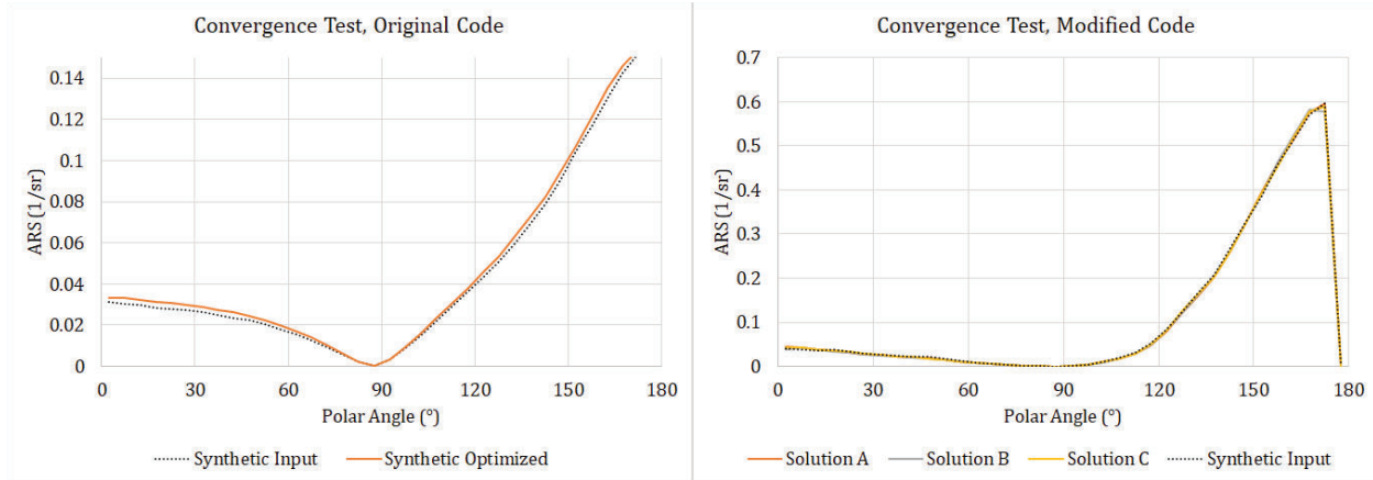
Figure 10. ARS datasets generated from MCSLinv convergence testing
