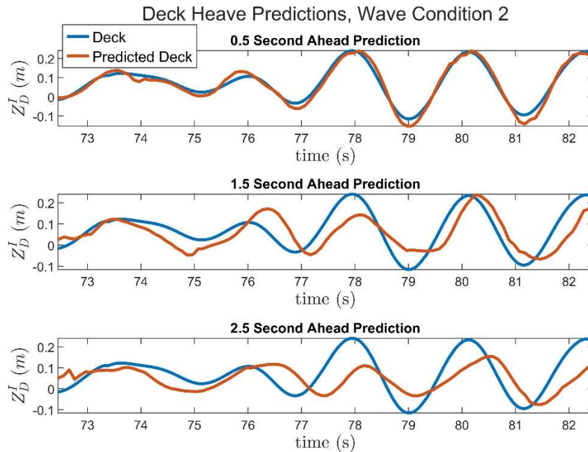
Figure 22: Model scale deck heave predictions.
