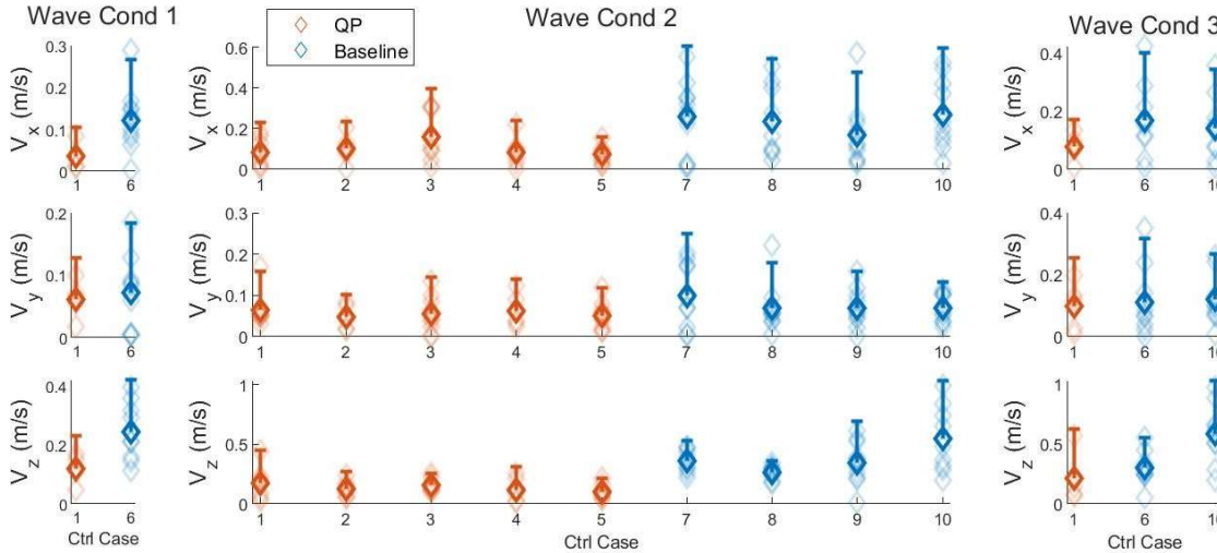
(b) Deck relative landing velocities.
