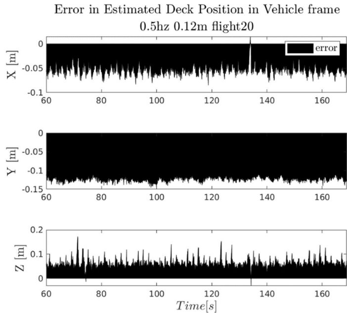
Figure 14: Sample plot of UKF position estimation error.
