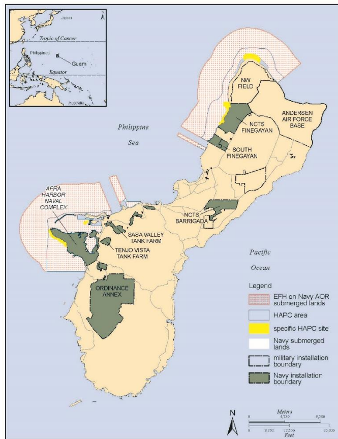
Figure 13. Navy Submerged Lands in Guam (PCR Environmental, 2007).
