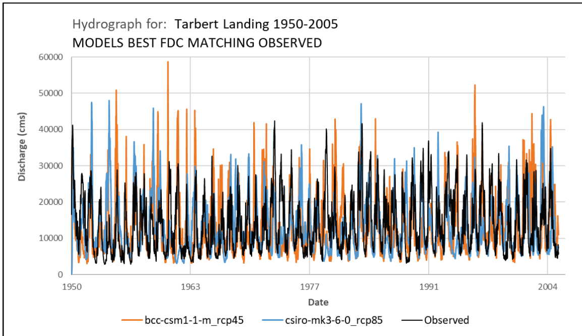
Figure 4. Hydrographs for the closest matching climate model FDCs (one match each for representative concentration pathway [RCP] 4.5 and RCP 8.5) to the FDC of the observed flow data for the period 1950–2005.
