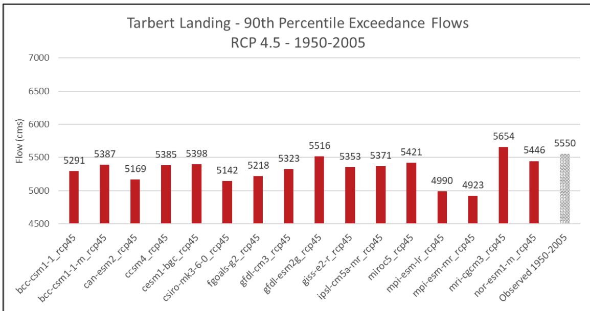
Figure 12. The 90th percentile exceedance flow values for RCP 4.5 based on data spanning 1950–2005.
