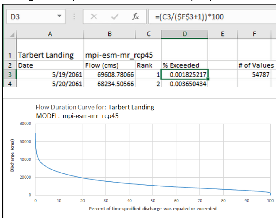
Figure 3. Example of how the flow duration curves (FDCs) were created.
