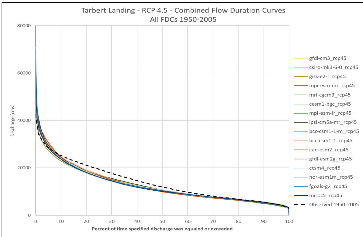
Figure 8. RCP 4.5, all climate model FDCs with the FDC for the observed flow data. All FDCs 1950–2005.
