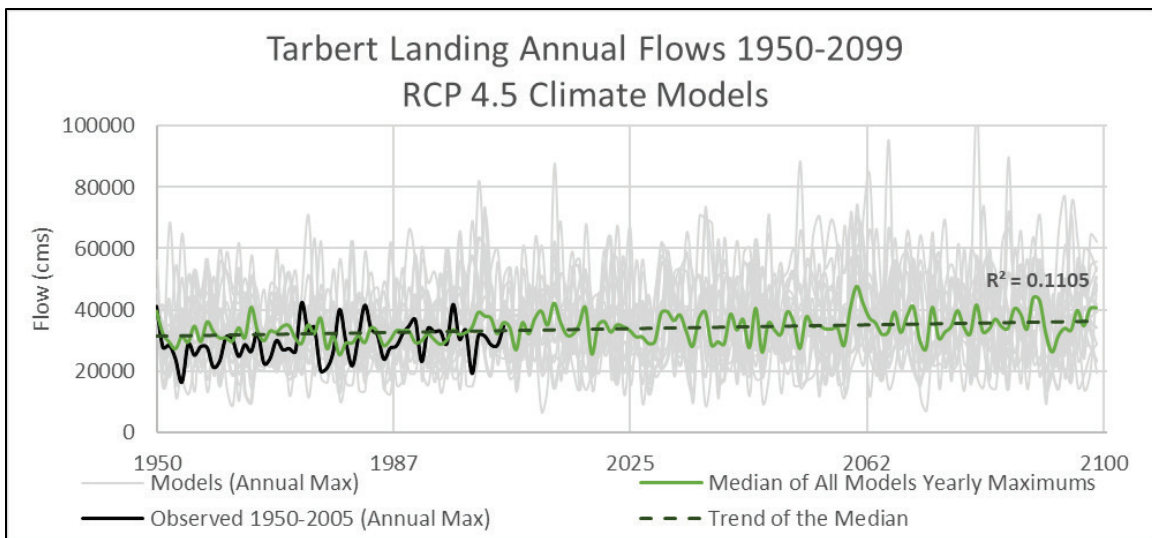
Figure 16. For the RCP 4.5 climate models—maximum annual flows and the median of the yearly maximum flows. The R^2 is for the trend of the median of all combined climate model flow results at Tarbert Landing for the RCP 4.5 scenario.
