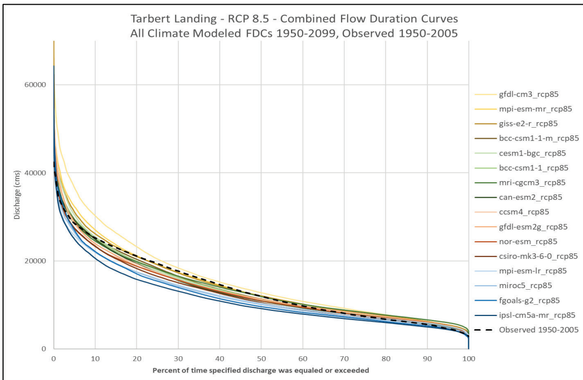
Figure 11. RCP 8.5, all climate model FDCs with the FDC for the observed flow data. All modeled FDCs 1950–2099. Observed 1950–2005.
