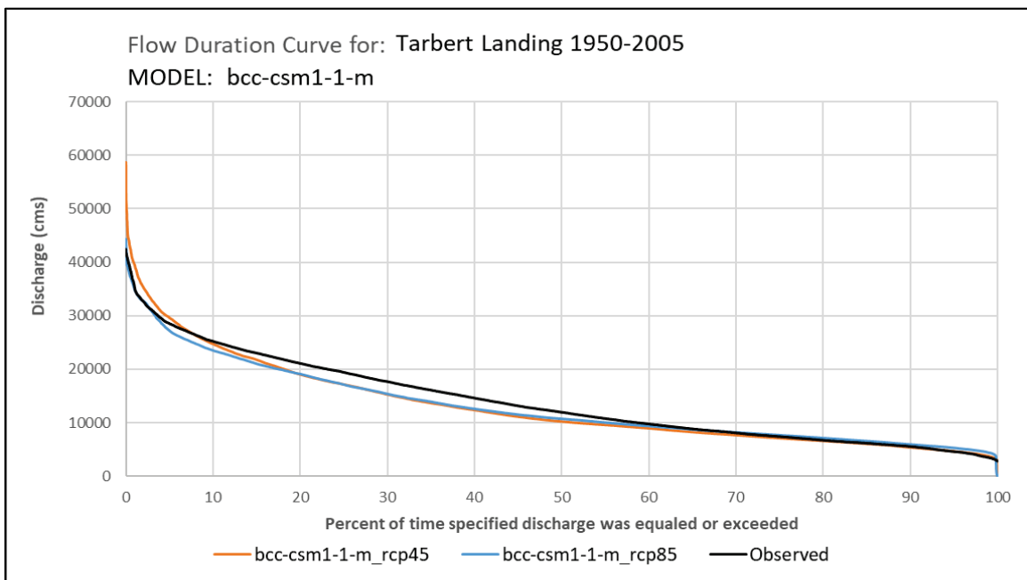
Figure 7. The climate model that most closely matched the observed flows for RCP 4.5 and RCP 8.5 together was bcc-csm1-1-m.
