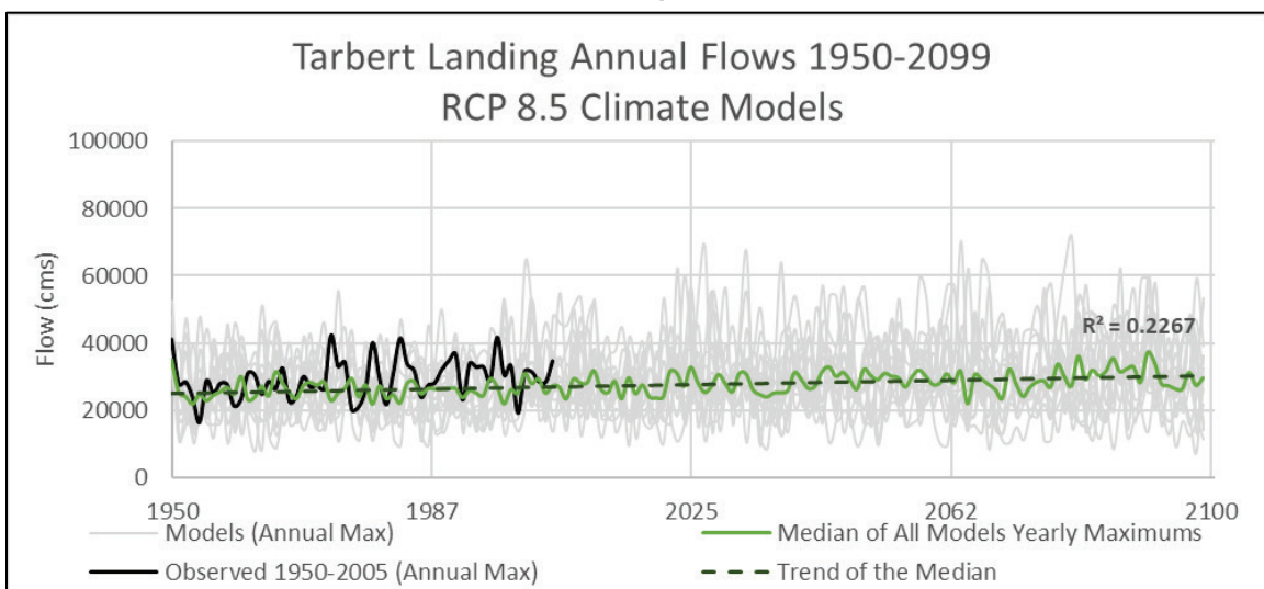
Figure 17. For the RCP 8.5 climate models—maximum annual flows, and the median of the yearly maximum flows. The R^2 is for the trend of the median of all combined climate model flow results at Tarbert Landing for the RCP 8.5 scenario.
