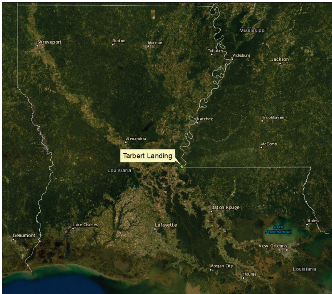
Figure 1. Location of Tarbert Landing.
