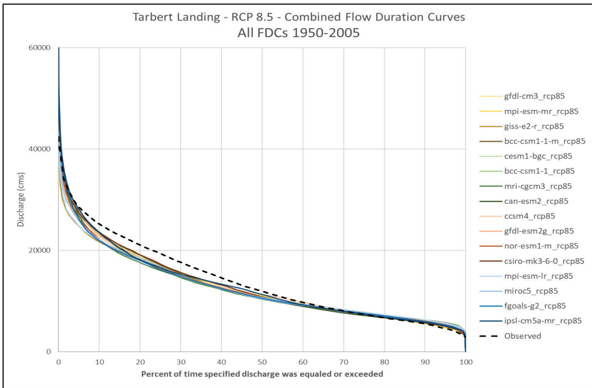
Figure 10. RCP 8.5, all climate model FDCs with the FDC for the observed flow data. All FDCs 1950–2005.
