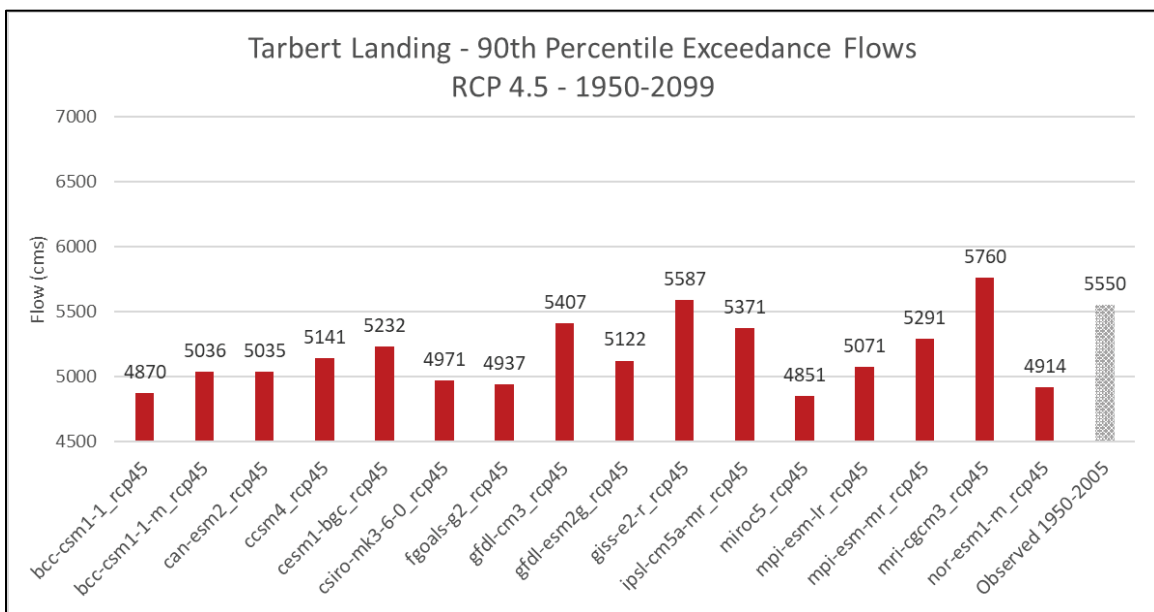
Figure 13. The 90th percentile exceedance flow values for RCP 4.5 based on data spanning 1950–2099.
