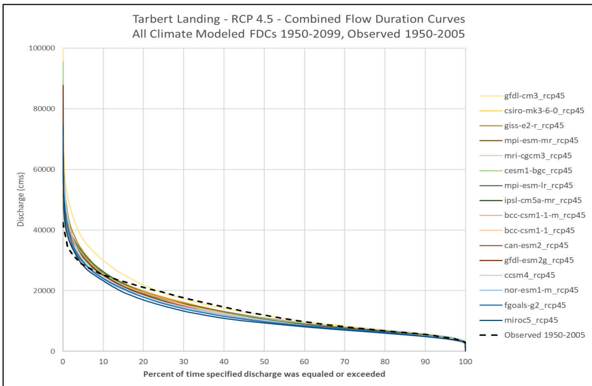
Figure 9. RCP 4.5, all climate model FDCs with the FDC for the observed flow data. All modeled FDCs 1950–2099. Observed 1950–2005.
