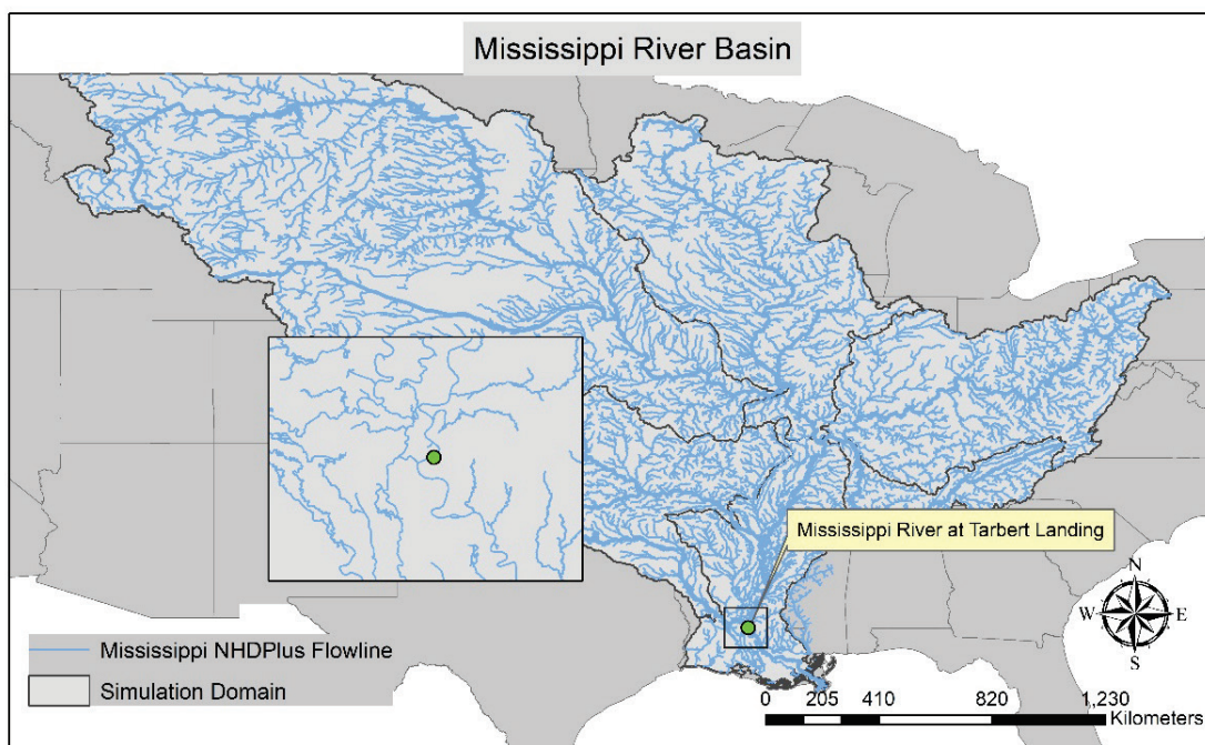
Figure 2. The Mississippi River Basin (MRB) and the Tarbert Landing location. The river network is produced based on the National Hydrography Dataset Plus (NHDPlus) dataset.
