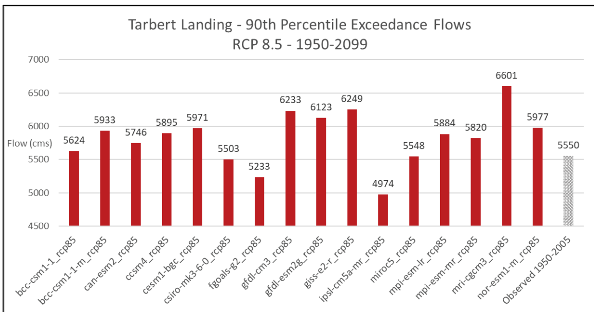
Figure 15. The 90th percentile exceedance flow values for RCP 8.5 based on data spanning 1950–2099.
