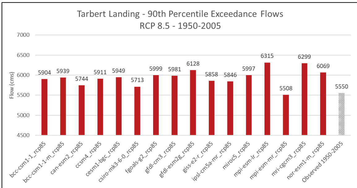
Figure 14. The 90th percentile exceedance flow values for RCP 8.5 based on data spanning 1950–2005.
