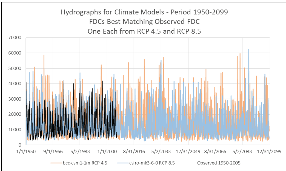
Figure 6. Hydrographs for the closest matching climate model FDCs (one match each for RCP 4.5 and RCP 8.5) to the FDC of the observed flow data for the period 1950–2099.
