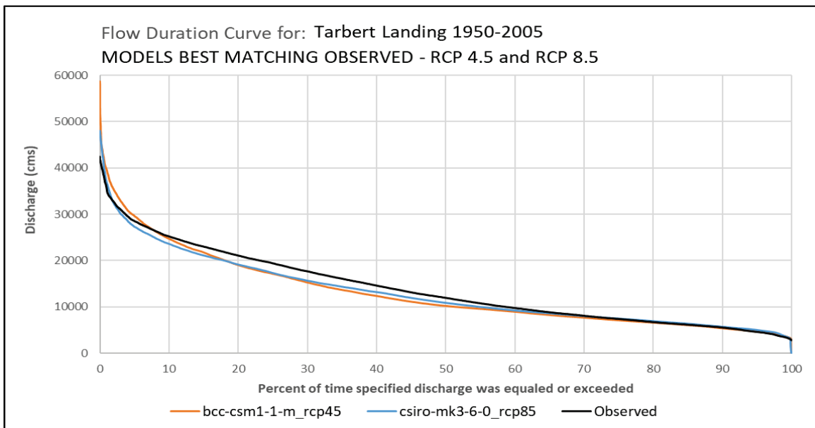
Figure 5. The closest matching climate model FDCs (one match each for RCP 4.5 and RCP 8.5) to the FDC of the observed flow data.
