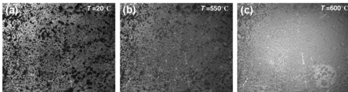
Figure 6. Recorded Images of the Surface of a Stainless Steel Sample Using a Conventional Optical Imaging System at Temperatures of (a) 20, (b) 550 and (c) 600 °C [66].
