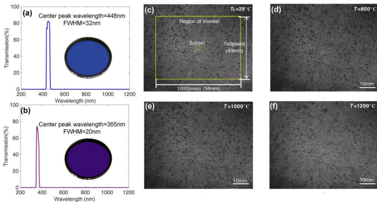
Figure 7. Transmission Spectrum of (a) a Blue Filter and (b) a UV Filter. Recorded Images of the Surface of a Stainless Steel Sample Using a Blue-light DIC System at Temperatures of (c) 28, (d) 800, (e) 1000 and (f) 1200 °C [66].
