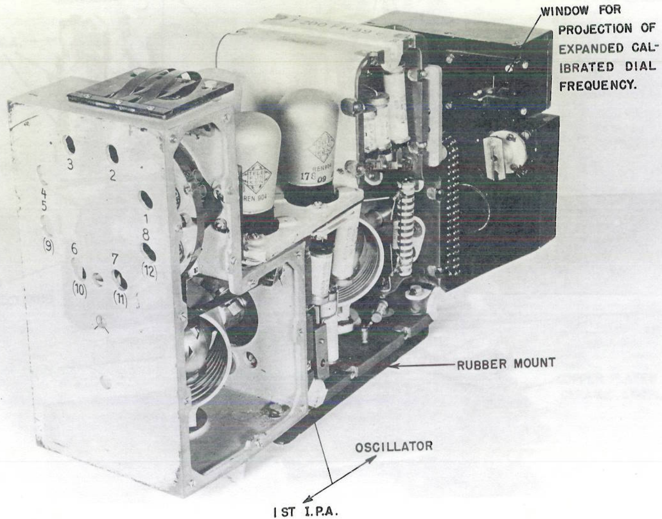
1st I.P.A. AND OSCILLATOR REMOVED FROM UNIT J - RIGHT FRONT.
