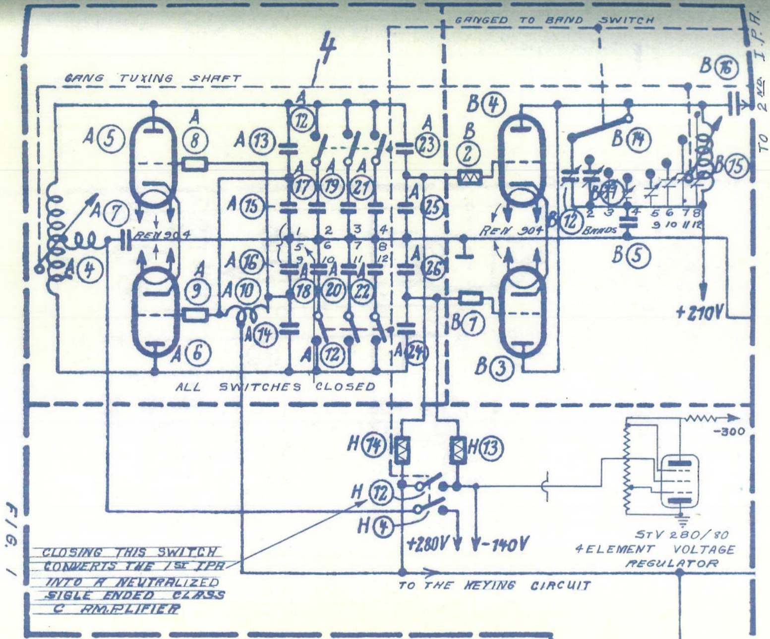
SCHEMATIC OF OSCILLATOR & 1st I.P.F.
