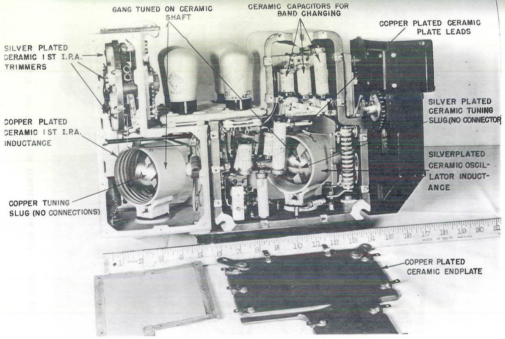
OSCILLATOR AND 1 st I.P.A. - RIGHT SIDE.
