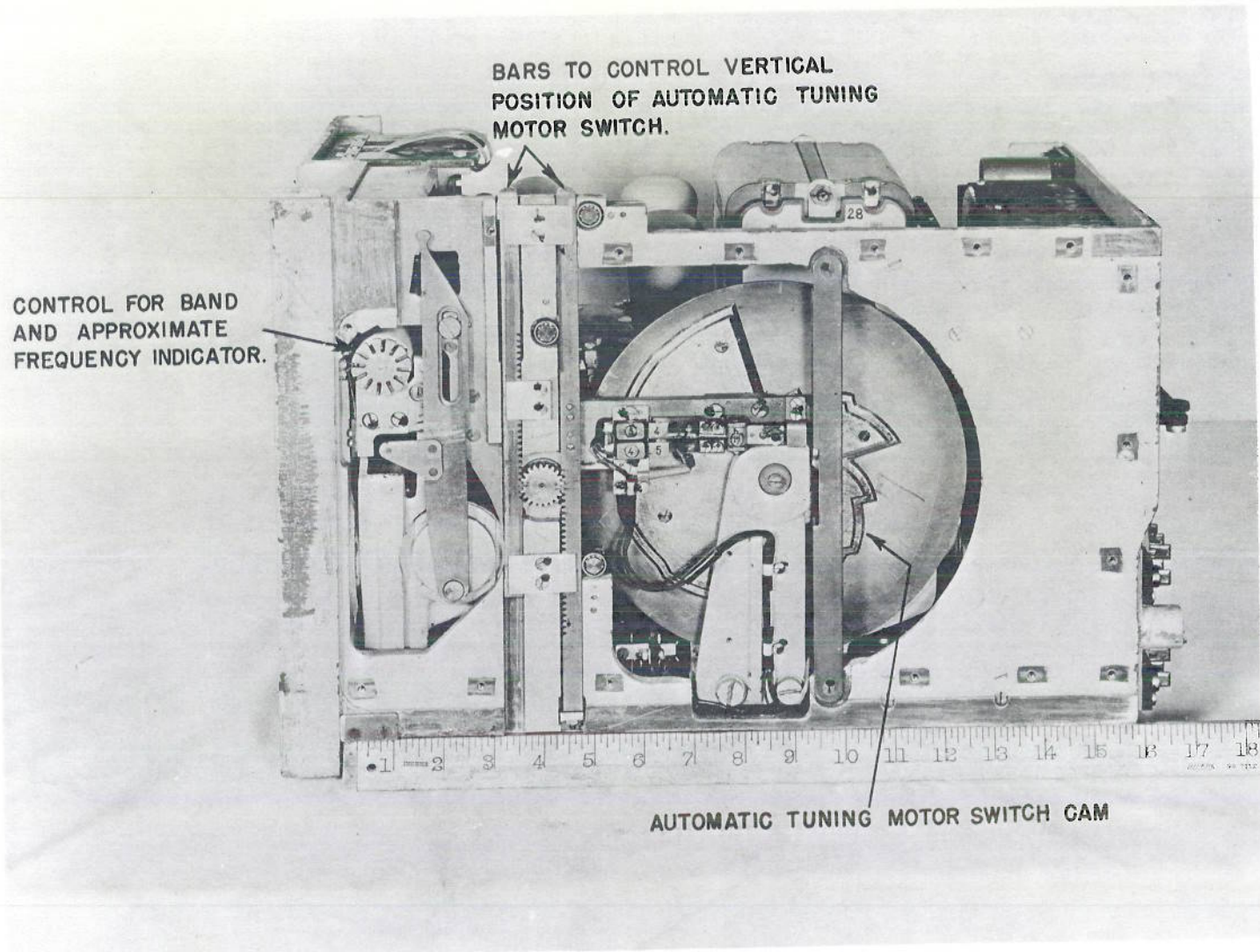
UNIT J - RIGHT SIDE, SHIELDS REMOVED.
