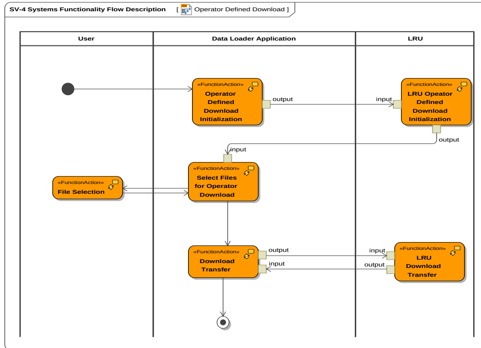
Figure 28. SVC-4 with Flow Description to Represent Logical View
