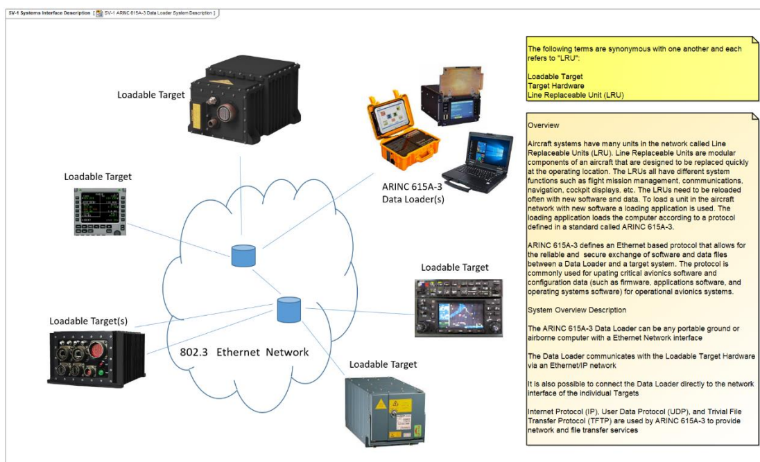
Figure 22. Operational Concept of the ARINC-615A Data Loader
