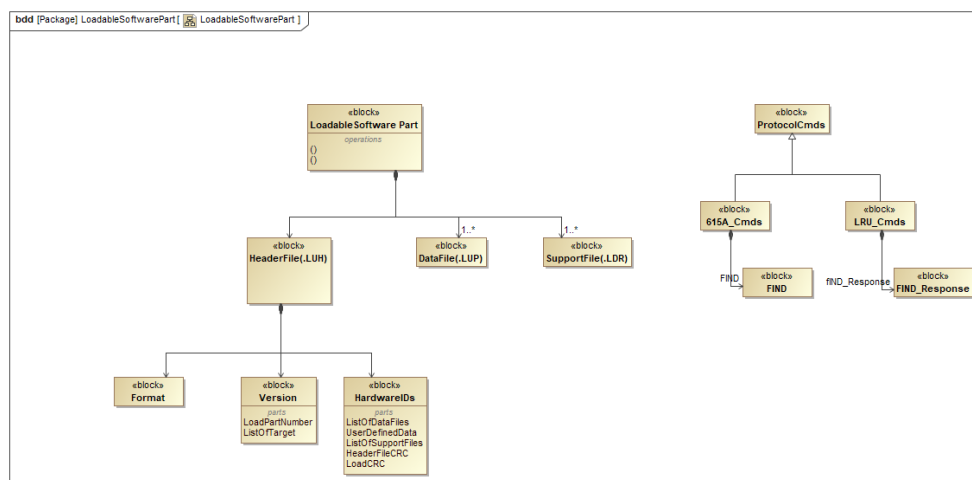
Figure 29. Data Submodel for the Data Loader (Partial)
