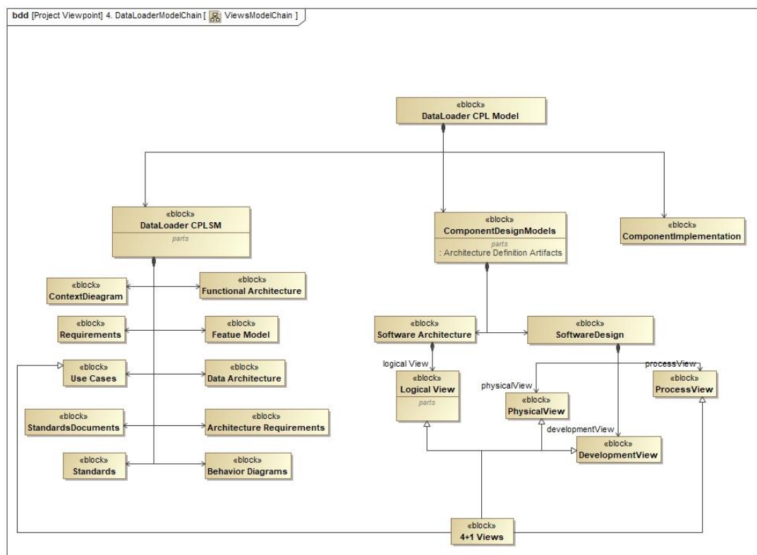
Figure 23. The Model Chain for the Data Loader
