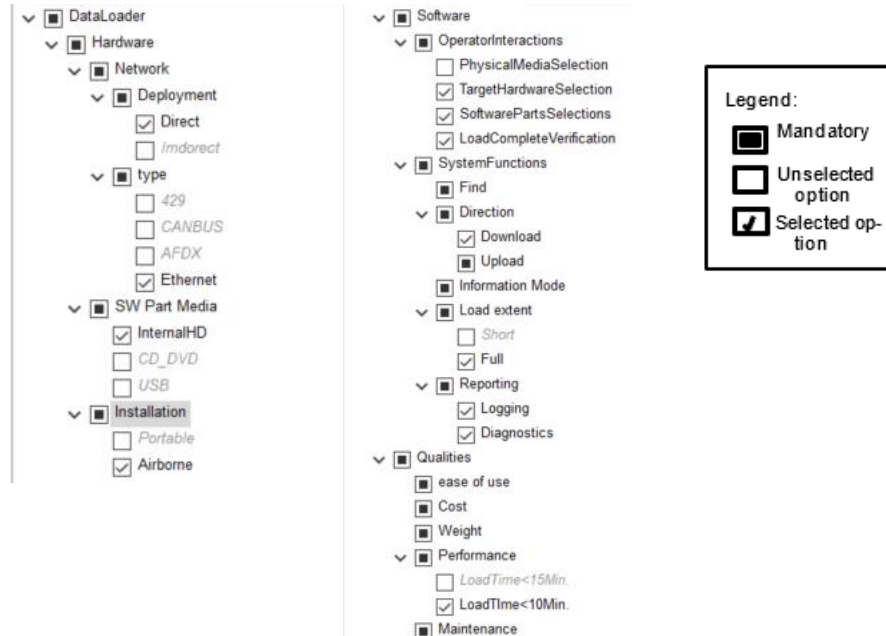
Figure 20. A Feature Set Derived from the Feature Model
