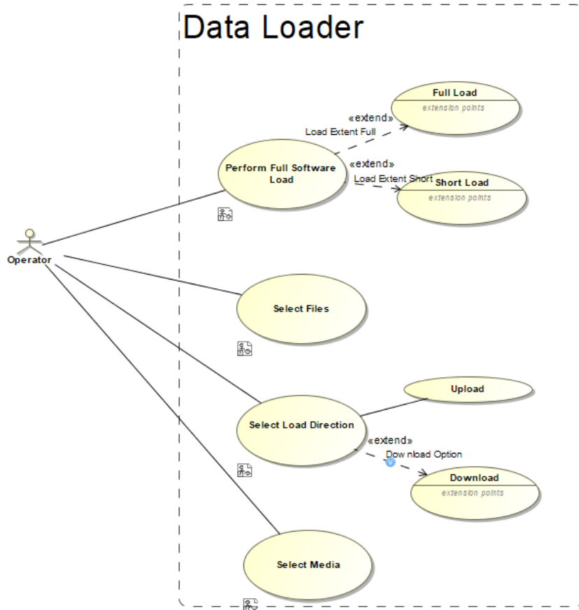
Figure 24. Use Cases from the Data Loader CPLSM
