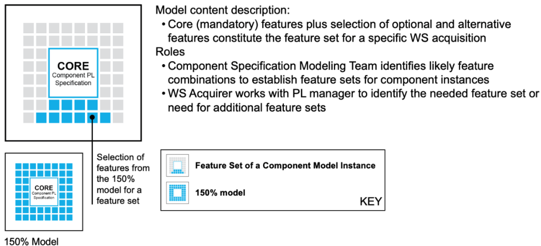
Figure 4. Component Instance (100%) Model – Selection of Core Features, Options, and Alternatives
