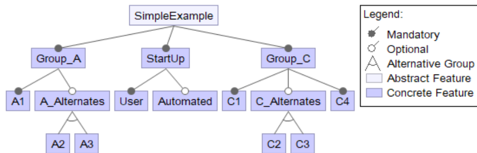
Figure 7. Feature Model Representation with Core and Variations
