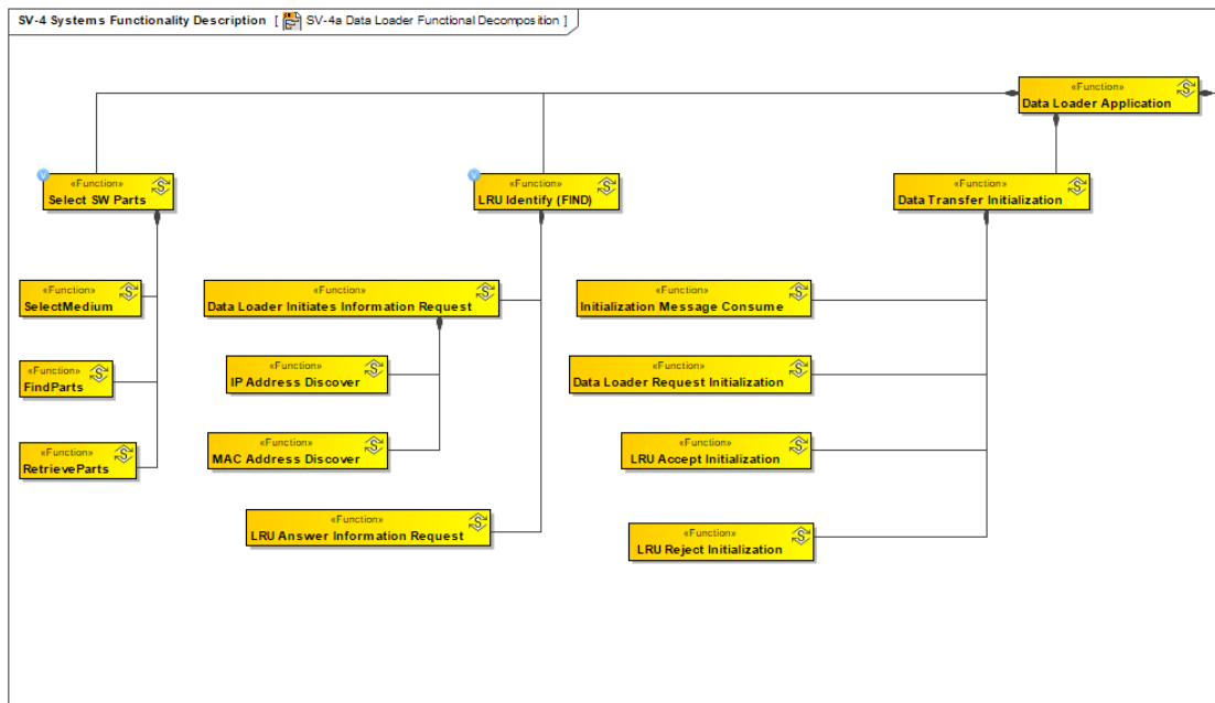
Figure 14. Use of SV-4 to Represent Functional Architecture (Hierarchy)
