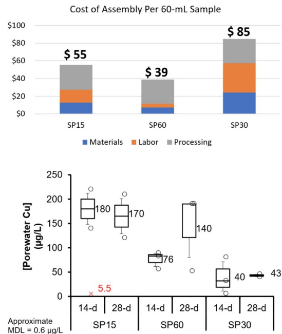
Figure 1: Example copper results shown above indicate that the SP15 peeper design provides an optimal balance in cost, sample volume, and equilibration speed (~14 days)
