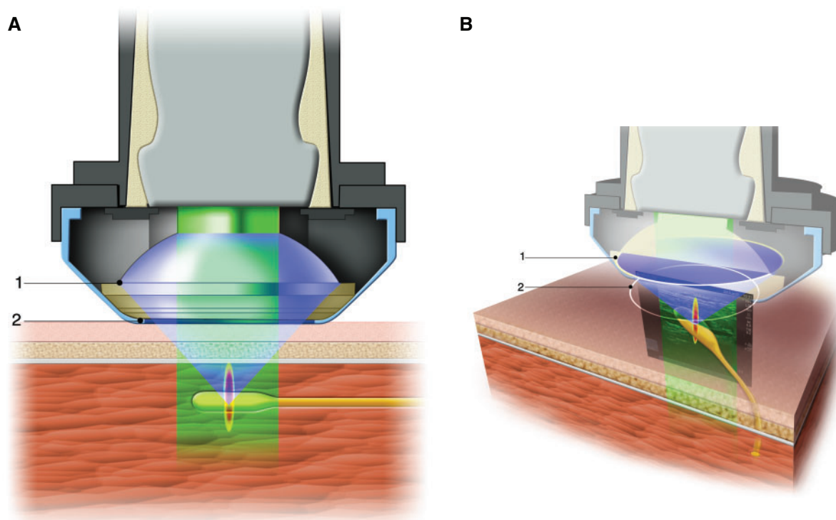
Figure 1 A) Illustration of the ig-iFU device focused on a horizontal cross-section of a neuroma. B) Illustration of the ig-iFU device focused on a neuroma, using a three-dimensional view of the device with a sample B-mode image placed within the image.
