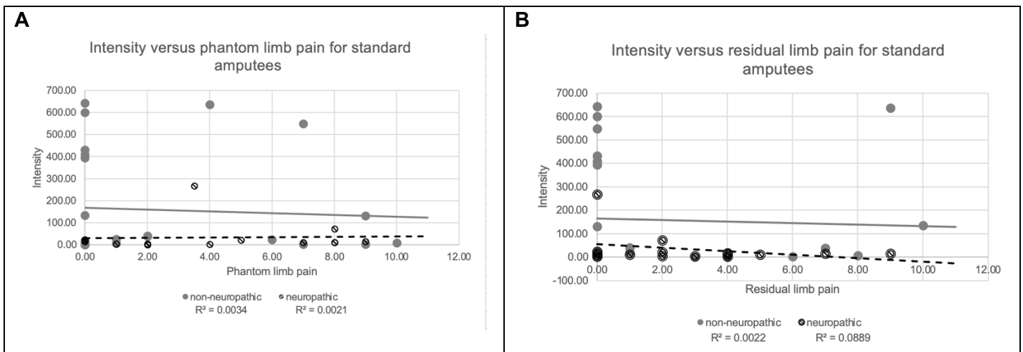
Figure 9. Intensity value necessary to create a sensation in a transected nerve of a standard amputee versus (A) phantom limb pain score and (B) residual limb pain score. Regression analysis examining phantom limb pain score versus intensity revealed no relationship across all standard amputation test subjects nor for neuropathic standard amputee test subjects alone. Data points with a line through them indicate test subjects deemed neuropathic via the LANNS pain score.
