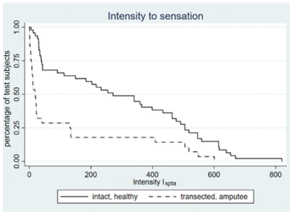
Fig. 8. Kaplan-Meier plots of intensity of ultrasound necessary to create a sensation for each of intact volunteers (intact nerves) and the transected nerves of participants with amputation. I_{\text{spta}} = spatial peak, temporal average intensity.
