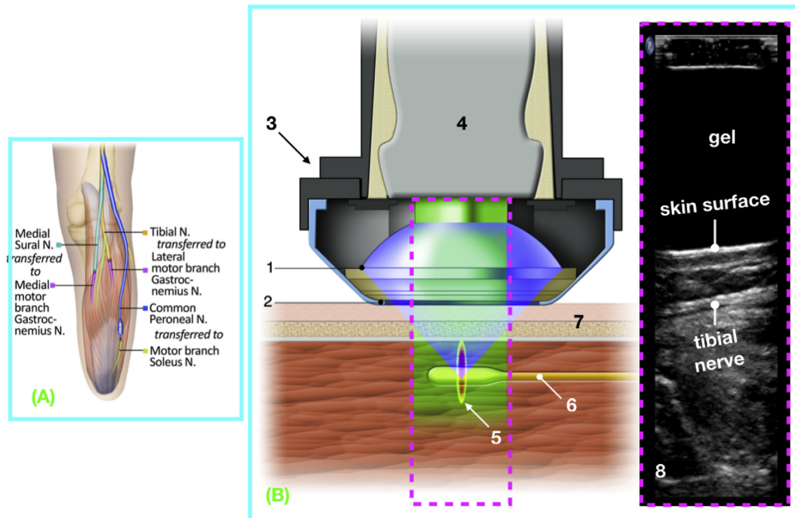
Fig. 1. Experimental target and setup. (A) Schematic of the test subject's major peripheral nerves in his residual limb. We targeted the distal aspect of the tibial nerve for stimulation by intense focused ultrasound. This schematic also shows the other nerves that had undergone the TMR procedure, with a neuroma at the distal end of the common peroneal nerve. (B) Schematic of the experimental procedure using an ultrasound system (#1 iFU transducer), 2 {gel pad, which couples the transducer to skin}, 3 {mounting system}, 4 {diagnostic ultrasound scan head}) that puts the ultrasound focus (#5) on the tibial nerve (#6) below the skin (#7) using ultrasound image guidance (#8).
