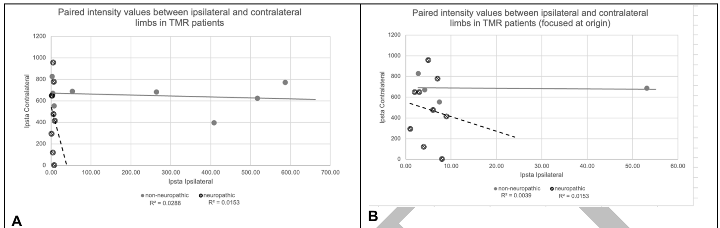
Figure 7 For TMR amputee test subjects, paired intensity values necessary to generate a discernable sensation (or maximum of the device) in transected (ipsilateral) and intact (contralateral) nerves.
