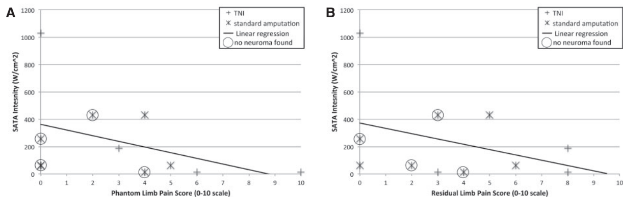
Figure 3 A) iFU threshold stimulation intensity value vs pain scores, each score rated over the last 24 hours: Intensity ( \text{w/cm}^2 SATA) vs phantom limb pain score (all data R^2 = 0.18 ). Neither inverse trend achieved statistical significance. B) iFU threshold stimulation intensity value versus pain scores, each score rated over the last 24 hours: Intensity ( \text{w/cm}^2 SATA) versus residual limb pain score (all data R^2 = 0.14 ). Neither inverse trend achieved statistical significance.
