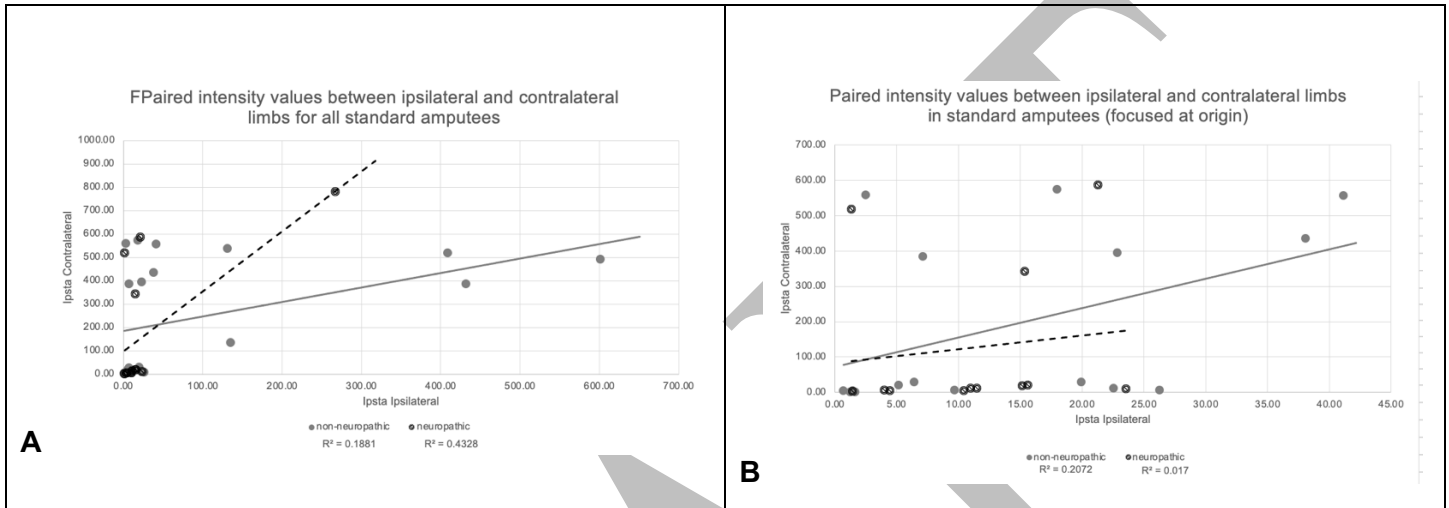
Figure 6. For standard amputee test subjects, paired intensity values necessary to generate a discernable sensation (or maximum of the device) in transected (ipsilateral) and intact (contralateral) nerves, (A) for all test subjects and (B) a close up of the data associated with the standard amputees most sensitive to ultrasound stimulation. (A) There was a significant difference in the intensity necessary to create a sensation for the intact versus paired transected nerve across all standard amputee test subjects. There exist a sub-set (B) of standard amputees that have comparable levels of sensitivity to iFU stimulation between their ipsilateral and contralateral limb. Data points with a line through them indicate test subjects deemed neuropathic via the LANNS pain score. Data point with a circle denotes data from a test subject with a neuroma. Note the large difference in range of the ipsilateral versus contralateral data points in Figures 6..
