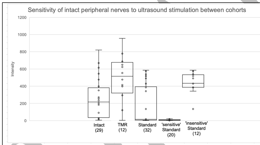
Figure 3: Sensitivity of intact peripheral nerves to ultrasound stimulation pooled across test cohorts. Intensity of ultrasound necessary to stimulate intact peripheral nerves of healthy participants and from the contralateral limb of standard and of TMR amputee participants. (We have divided the data from standard amputees into two subgroups – one very sensitive to IFU and one insensitive to iFU.)
