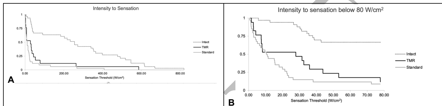
Figure 5: Kaplan-Meier plots of intensity of ultrasound necessary to create a sensation for each of intact test subjects (intact nerves) and the transected nerves of standard amputees and TMR amputees. (A) Shows a display of all the data while (B) displays the data associated with intensity values below 80 W/cm 2 .
