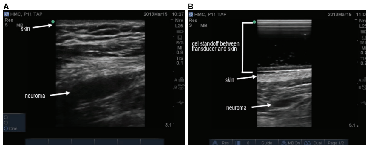
Figure 2 A) Sample B-mode ultrasound image of a neuroma captured directly with the Sonosite ultrasound imaging device. B) Sample B-mode ultrasound image of a neuroma with the Sonosite device placed within the ig-iFU system.
