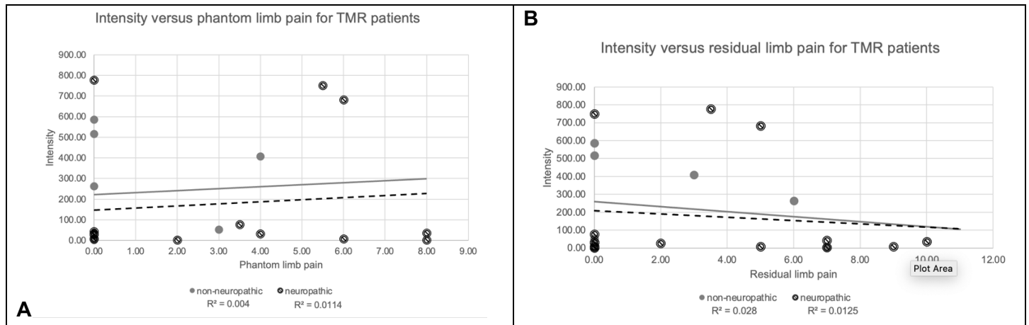
Figure 10. Intensity value necessary to create a sensation in a transected nerve versus (A) phantom limb pain score and (B) residual limb pain score for all TMR amputees. (A) Linear regression analysis examining phantom limb pain and intensity revealed no relationship across all TMR amputation test subjects nor for neuropathic TMR test subjects only. Similarly, (B) linear regression analysis examining residual limb pain and intensity revealed no relationship across all TMR amputation test subjects nor for neuropathic TMR test subjects only. Data points with a line through them indicate test subjects deemed neuropathic via the LANNS pain score. Data points with circles identify individuals with neuromas.
