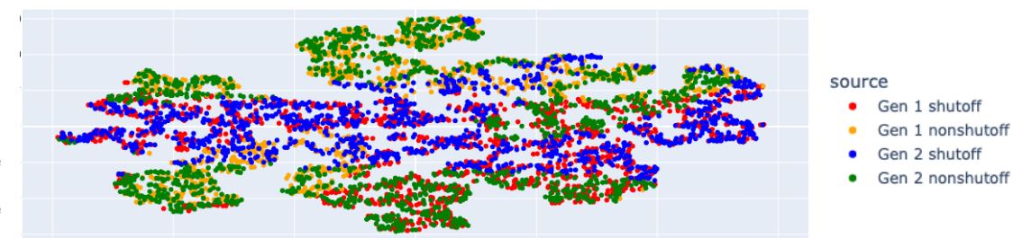
Figure 25. t-SNE TIP-GAN ( n=2 ) generator embeddings Timestep 20.
