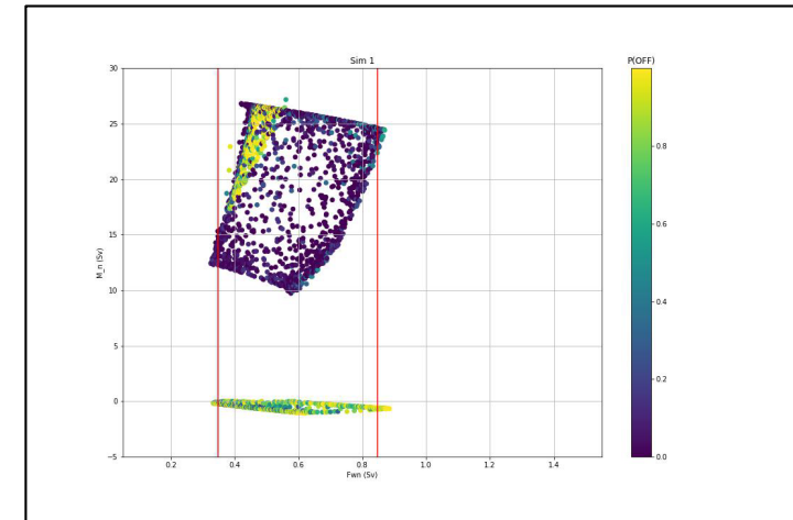
Figure 22. TIP-GAN with the inclusion of recovery labeling.
