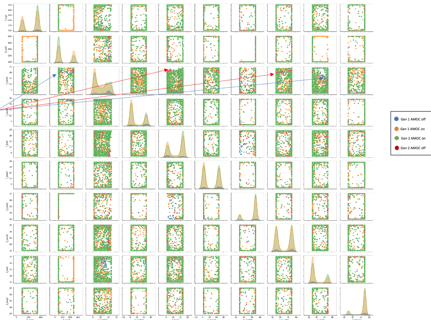
Figure 31. Shows a pair plot of CESM2 model parameters for understanding relationships between pairs of parameters.
