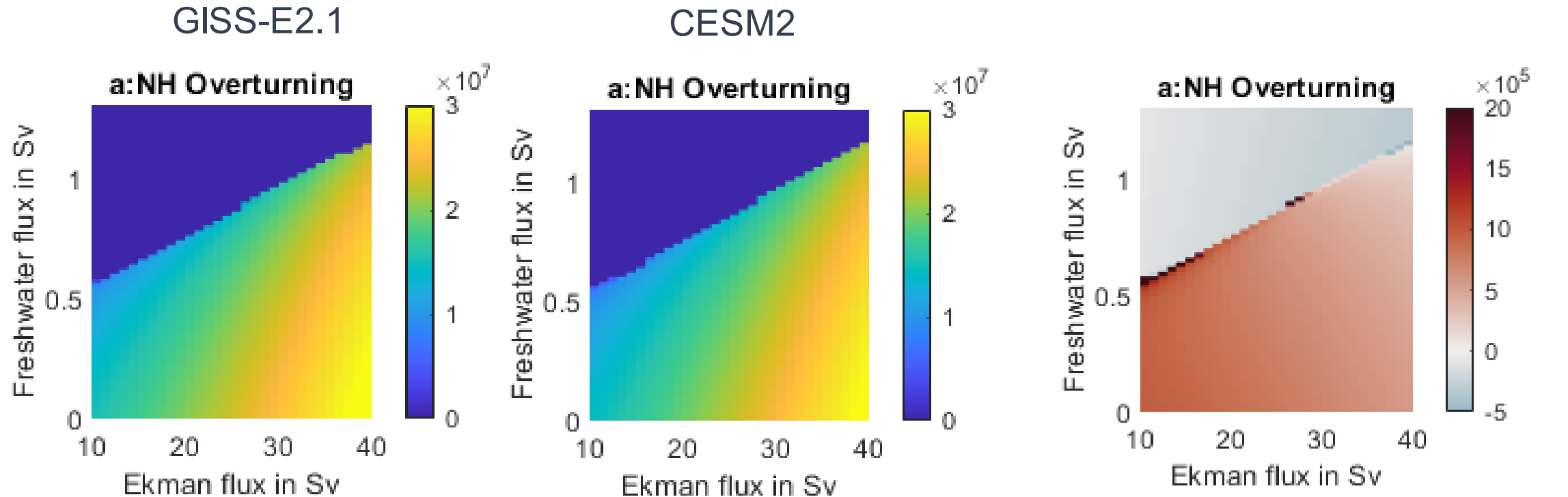
Figure 8. GISS and CESM2 as a function of Ekman flux and Freshwater flux.
