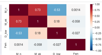
Figure 35. Generator 1 Pair plot and correlation plot of Four box model at end timestep.
