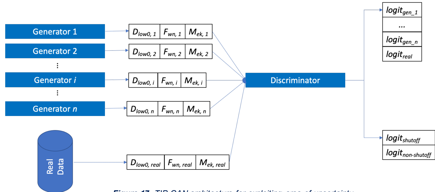
Figure 17. TIP-GAN architecture for exploiting area of uncertainty.
