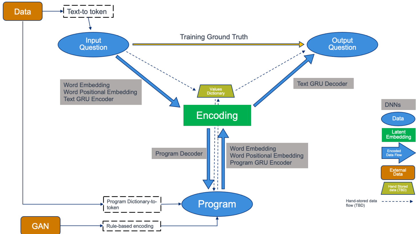
Figure 38. Neuro-symbolic translation questions to programs for GAN consumption and GAN output to NL questions for human consumption – *first of its kind*
