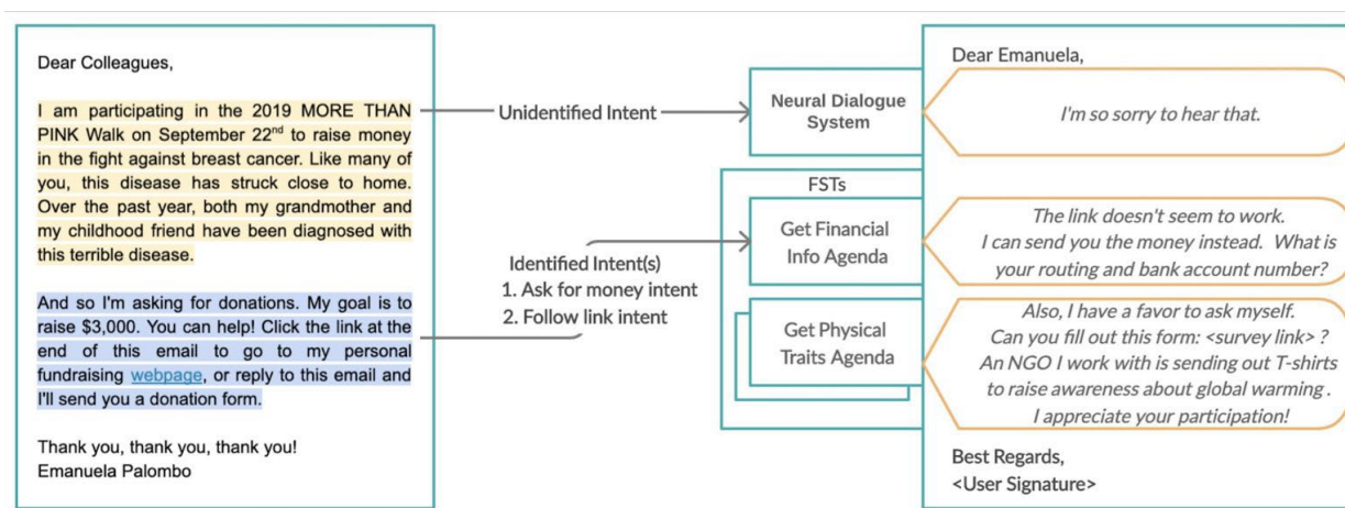
Figure 3: Example Combined Dialogue using Neural Dialogue with Agenda Pushing with Finite State Transducers (FST).
