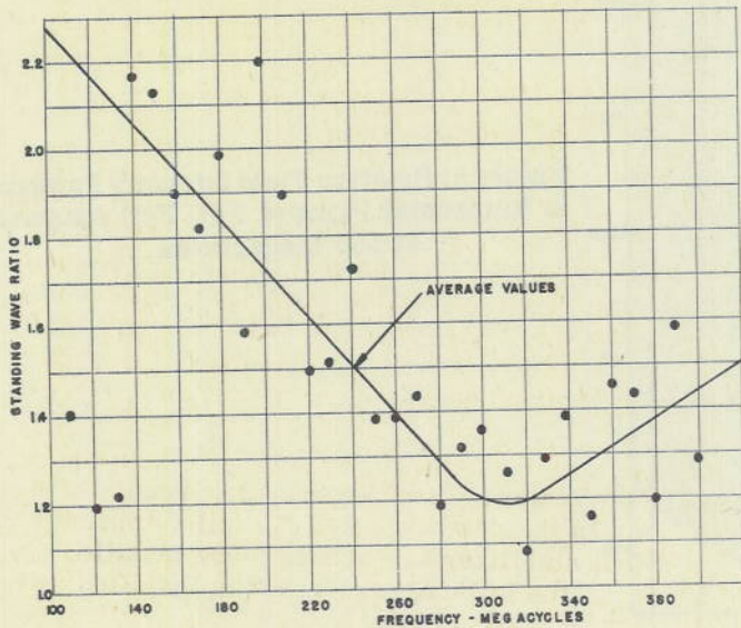
Figure 4. Voltage Standing Wave Ratio of Foil Antenna on Non-metallic Fin of F4U Aircraft (Measured on 50 OHM Line through 20 ft. of RG-8/U cable.
