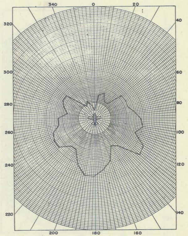
Figure 9. Relative Field Intensity Pattern in Horizontal Plane of F4U Foil Antenna at 400 megacycles
