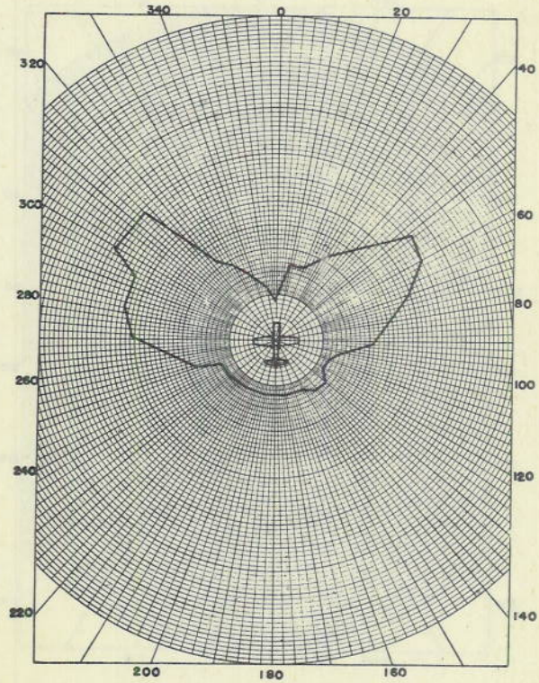
Figure 6. Relative Field Intensity Pattern in Horizontal Plane of F4U Foil Antenna at 235 megacycles
