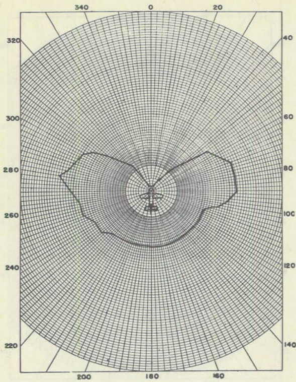
Figure 8. Relative Field Intensity Pattern in Horizontal Plane of F4U Foil Antenna at 314 megacycles
