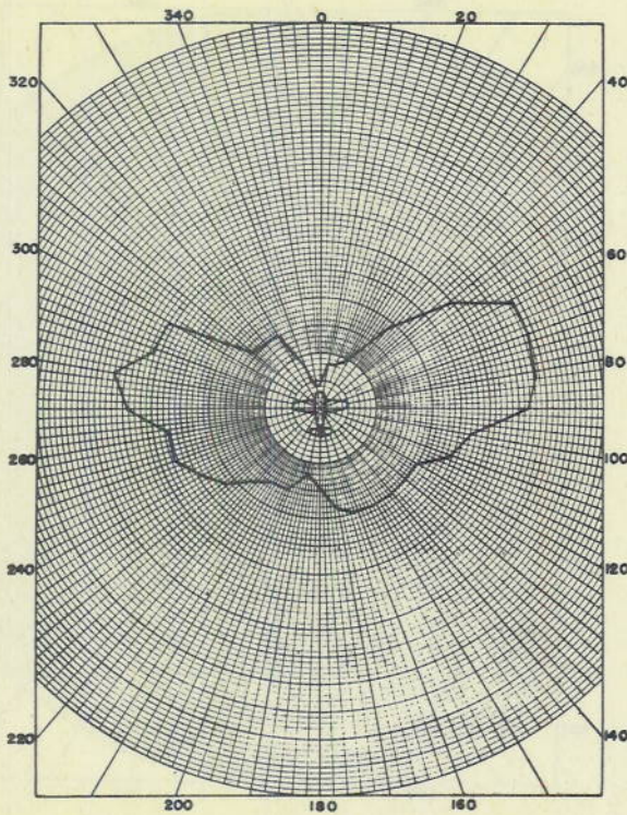
Figure 7. Relative Field Intensity Pattern in Horizontal Plane of F4U Foil Antenna at 293 megacycles
