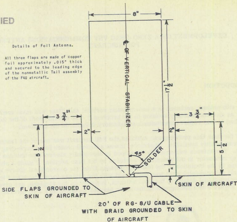
Figure 2. Details of Foil Antenna
