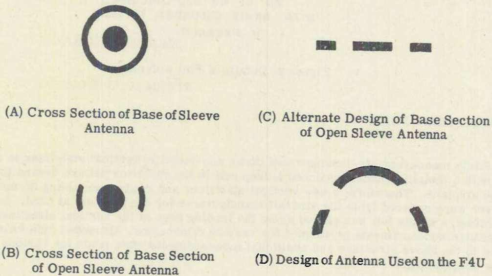
Figure 1. Development of the F4U Antenna from Sleeve Antenna
