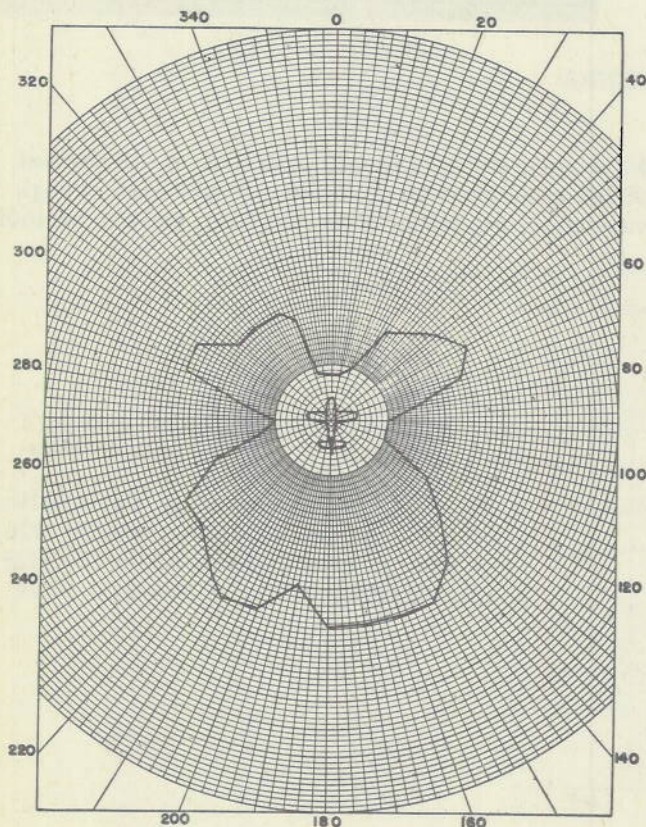
Figure 5. Relative Field Intensity Pattern in Horizontal Plane of F4U Foil Antenna at 136 megacycles
