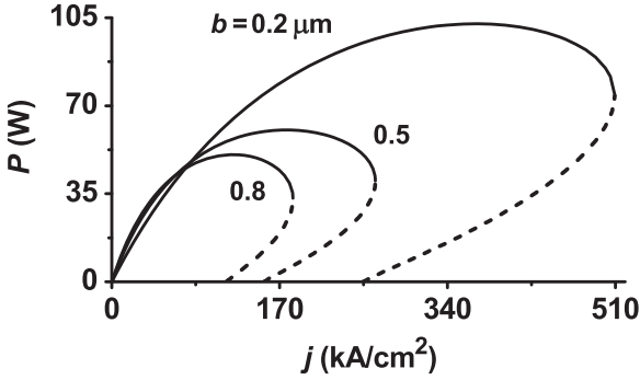
Fig. 6. Light-current characteristics for the structures with the OCL thicknesses b = 0.2, 0.5 , and 0.8 \mu\text{m} .
