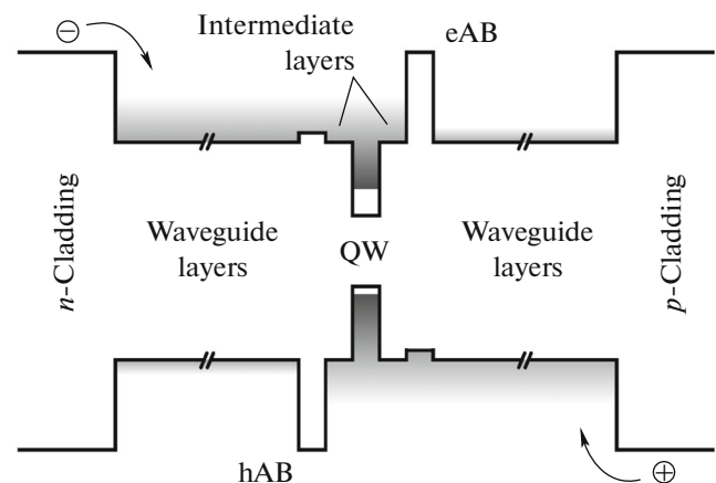
Fig. 1. Schematic energy band diagram illustrating the concept of a laser with ABs; p(n) -side AB [marked as eAB (hAB)] aims to suppress the electron (hole) transport.
