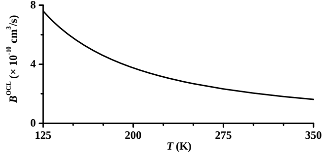
Fig. 1. Spontaneous radiative recombination constant for the OCL vs. temperature.
