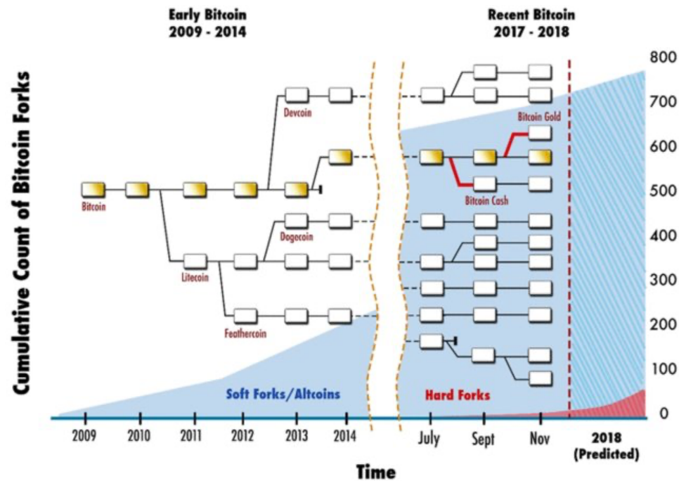
Figure 12 – Blockchain forks 39
