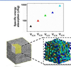
Atomic Scale Structure Inspired 3D-Printed Porous Structures with Tunable Mechanical Response, Adv. Eng. Mater. , 23: 2001428., 2021
