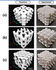
Flexure resistant 3D printed zeolite-inspired structures, Additive Manufacturing , 47, 2021, 102297
