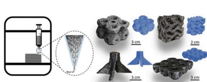
Three-dimensional printing of complex graphite structures, Carbon , 181, 2021, 260-269
