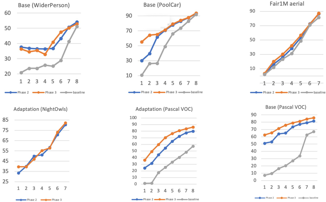
Figure 25. Performance graphs for phases 2, 3 of our system and the baseline (JPL) system, for some of the development datasets.
