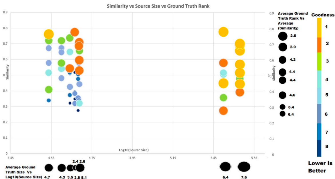
Figure 14. Relationship of performance of the target model to size of the source dataset (X-axis) and its similarity with source dataset (Y-axis) for 9 targets over 8 sources
