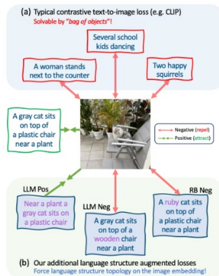
Figure 11. An illustration of our method for text augmentations to improve SVLC understanding.
