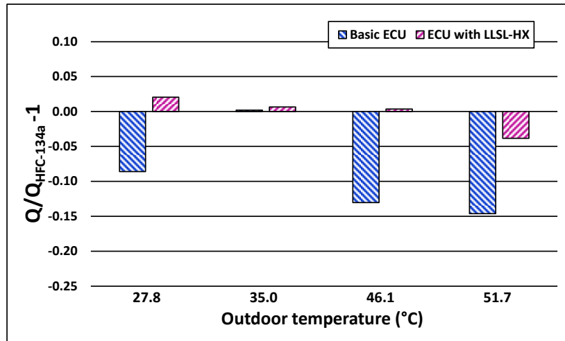
Figure 4.8-5. Capacity difference of CO 2 in basic ECU and ECU with LLSL-HX versus capacity of HFC-134a, referenced to HFC-134a capacity, for ECU with capacity matching that of HFC-134a at the 35.0 °C test condition; based on ACSIM.CO 2 simulations at outdoor temperatures 27.8 °C, 35.0 °C, 46.1 °C, and 51.7 °C
