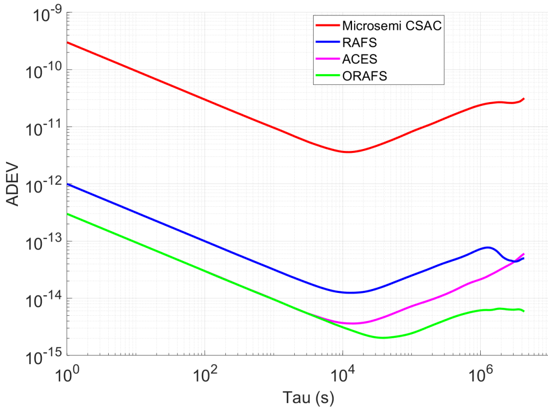
Figure 10. OADEVs of Various Simulated Clocks
