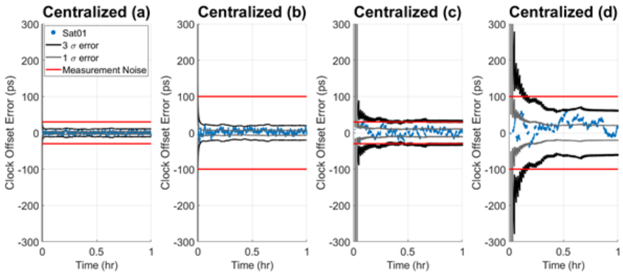
Figure 18. Time transfer error for a single satellite using a centralized estimation architecture. From left to right: a) 1s measurement rate, 30ps noise b) 1s measurement rate, 100ps noise, c) 60s measurement rate, 30ps noise, d) 60s measurement rate, 100ps noise
