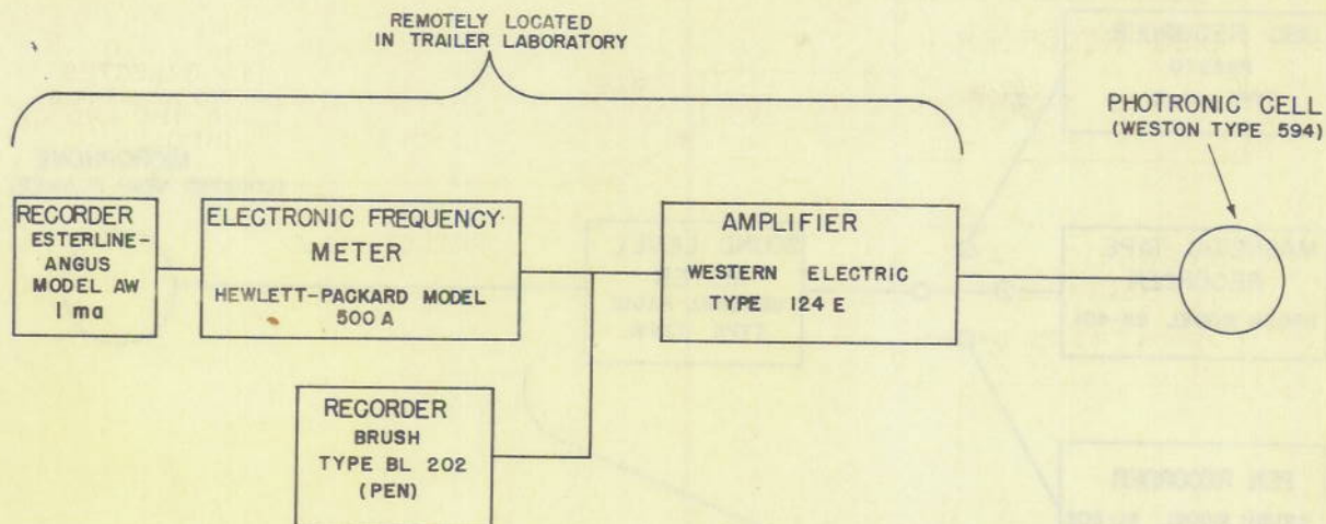
Figure 8 - Light Intensity vs. Time Instrumentation
