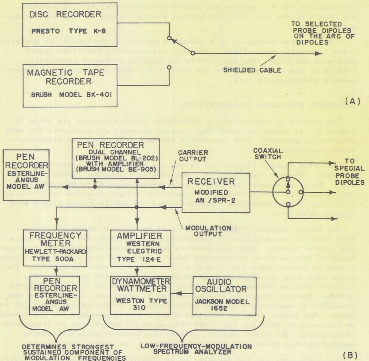
Figure 7 - Incidental Modulation Instrumentation
