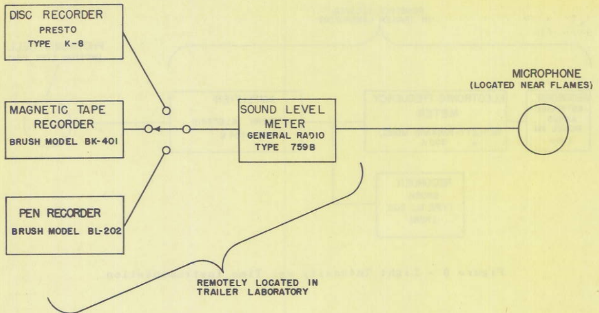
Figure 9 - Sound Field Instrumentation Showing Choice of Outputs
