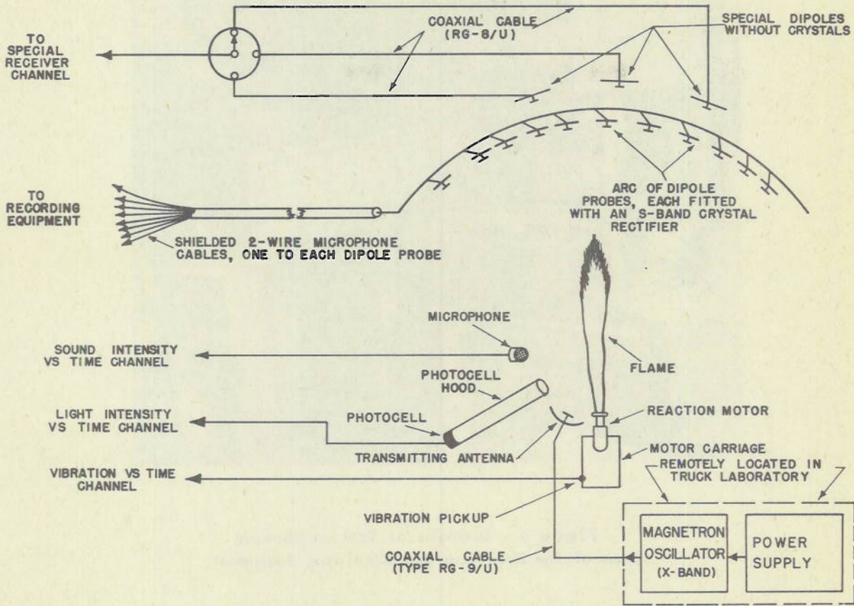
Figure 2 - Simplified Diagram of Incidental Modulation Observation Channels
