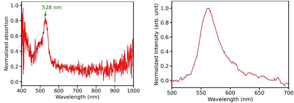
Fig 3: Absorption (left), emission (right) spectra of the aerosol formed with Rhodamine 6G.
