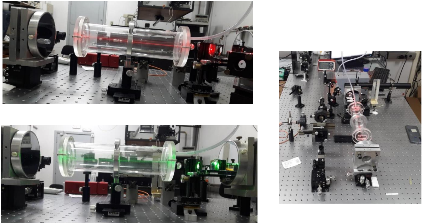
Fig. 8: Herriott-cell using a He-Ne laser (at 630 nm) (top left), Herriott-cell with the 2nd Harmonic Nd-YAG (at 532 nm) laser (bottom left) and top view of the set up (right).
