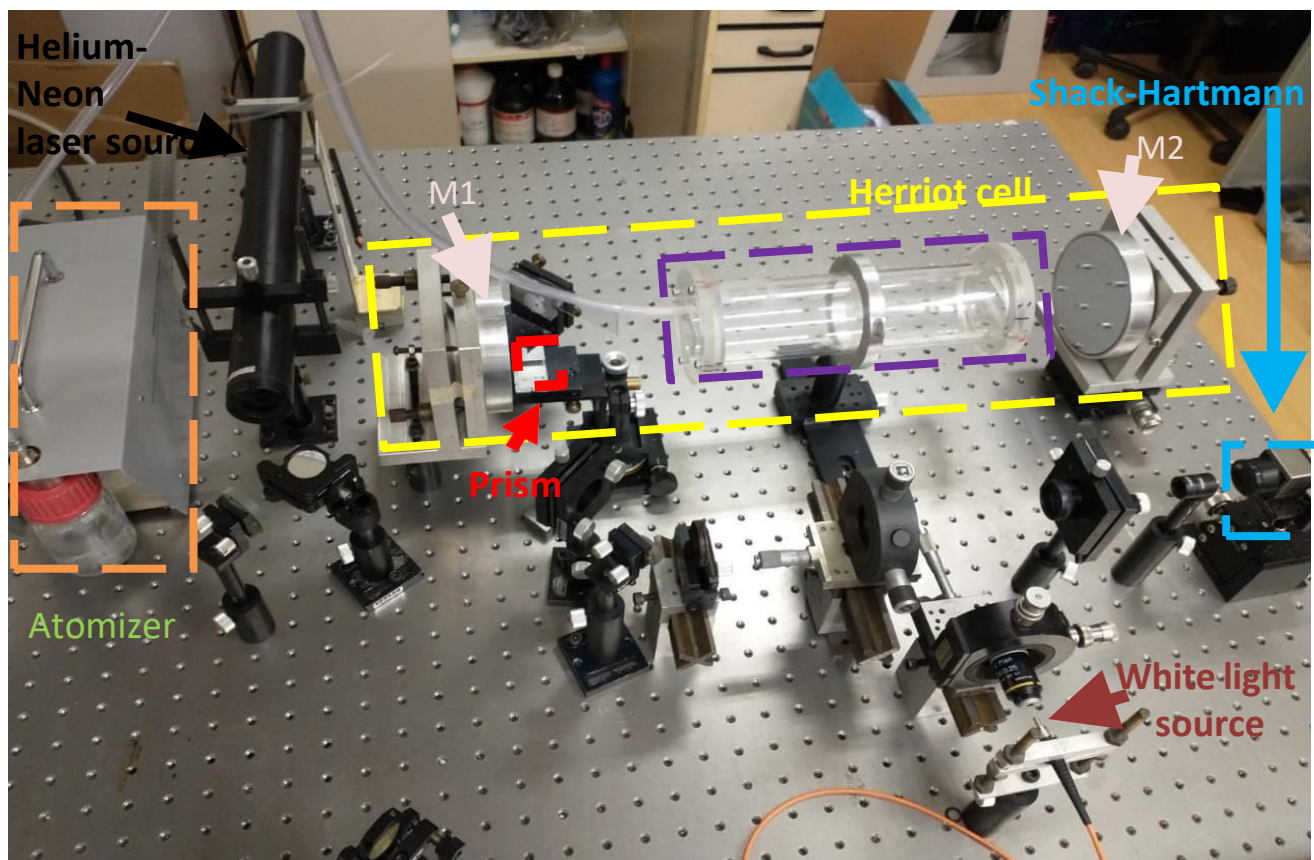
Fig. 7: Experimental set up for the generation and measurement of the nonlinear characteristics of the de Au nanorods aerosol mounted at PUC-Rio.
