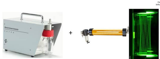
Fig1: Aerosol Generator (left)), Herriot Cell (right).
