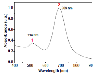
Fig. 6: Au nanorods absorption spectra as a function wavelength showing the typical LSPR absorption bands (left), and an image of the sample (right).
