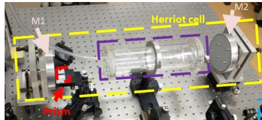
Fig 5: Home-made Herriot Cell(yellow dashed line): 2 concave mirrors (M1 and M2) and-prism (red dashed line).
