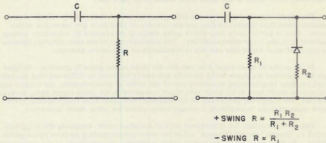
Fig. 5 - Conventional differentiator and modified differentiator circuits
