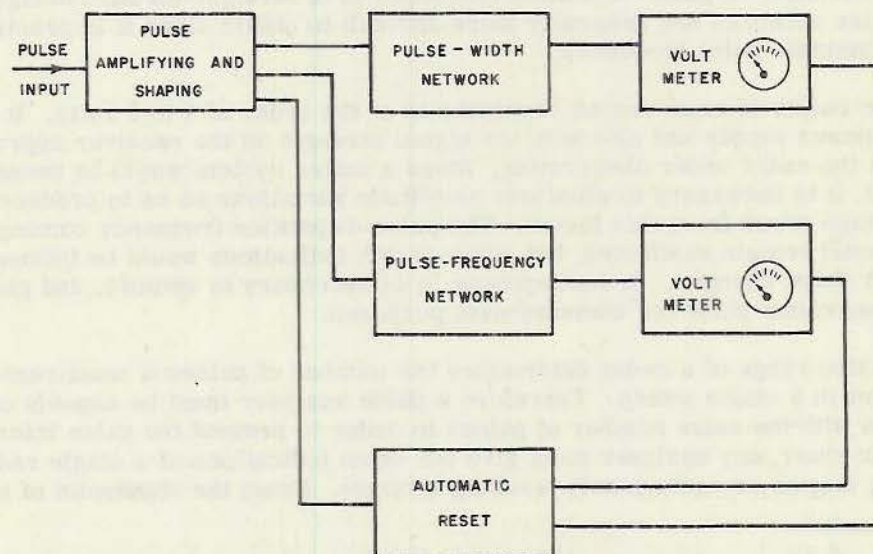
Fig. 1 - Basic block diagram of pulse analyzer
