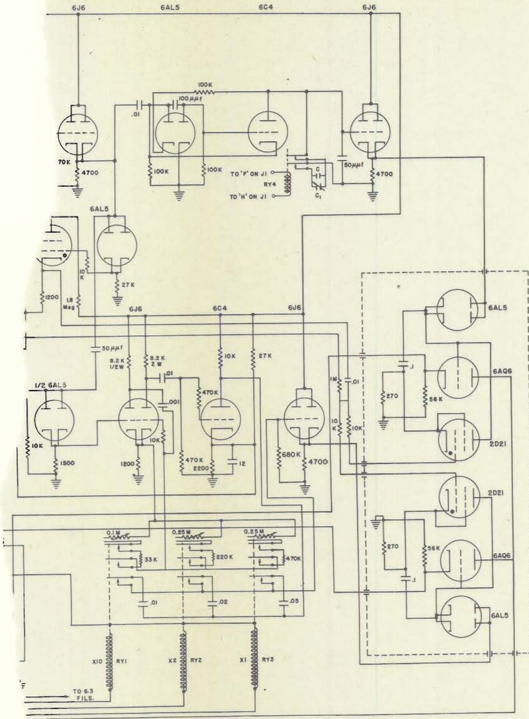
Fig. 2 - Schematic diagram APA-64 pulse analyzer
