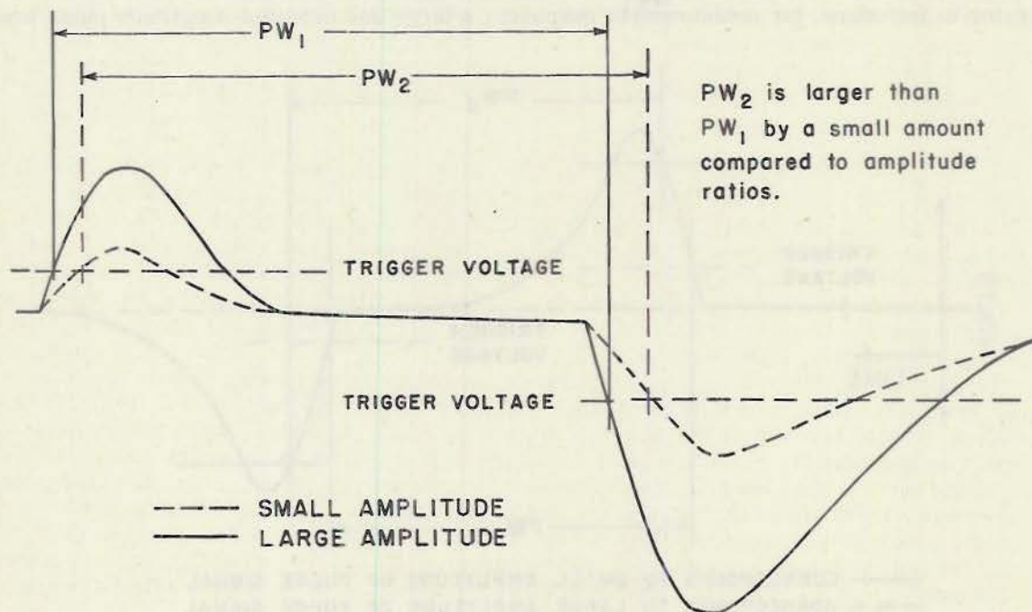
Fig. 6 - Differentiated square pulse from modified differentiator circuit
