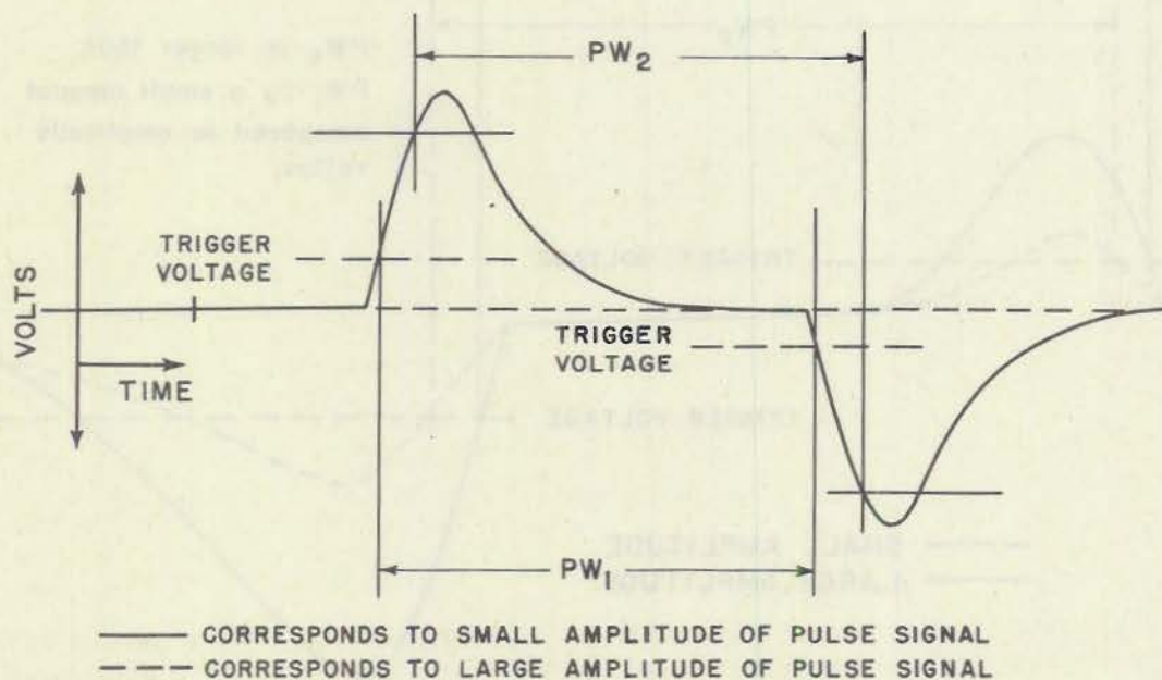
Fig. 4 - Differentiated square pulse
