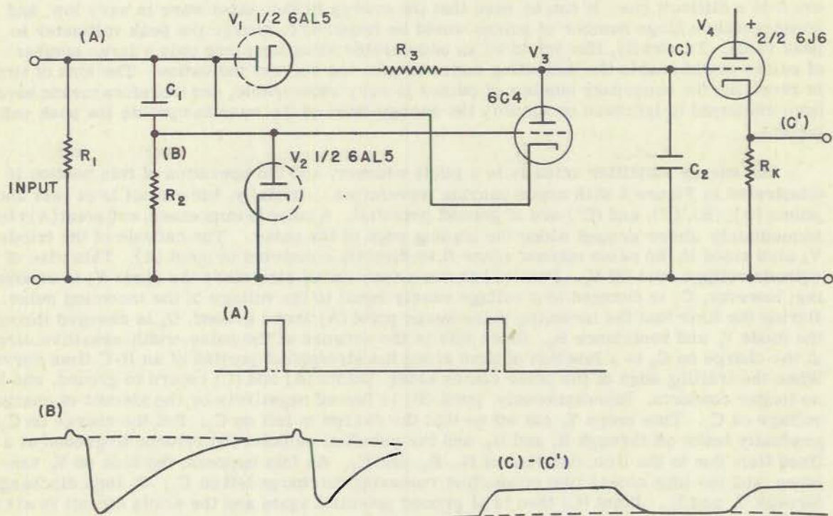
Fig. 8 - Pulse width network and energy amplifier with waveforms at important points
