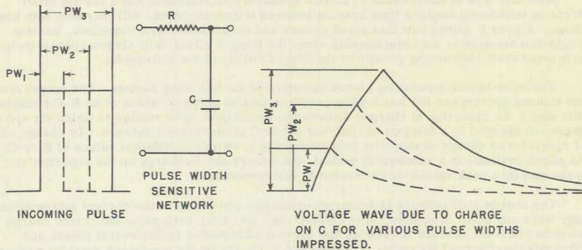
Fig. 7 - Integration of a square pulse
