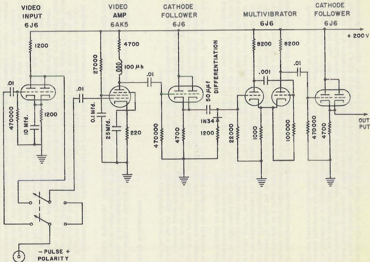
Fig. 3 - Schematic diagram, pulse amplifier and shaper
