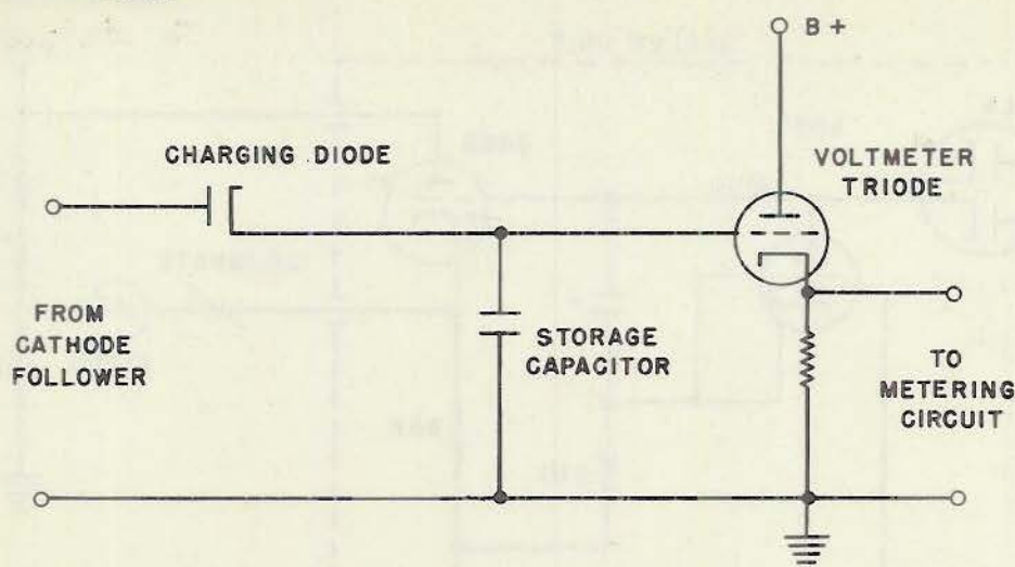
Fig. 12 - Basic voltmeter circuit
