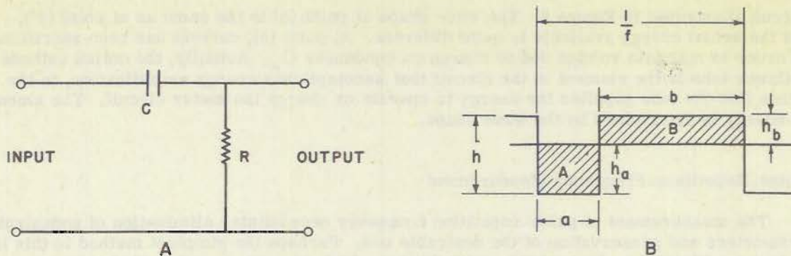
Fig. 9 - Averaging circuit and waveform diagram
