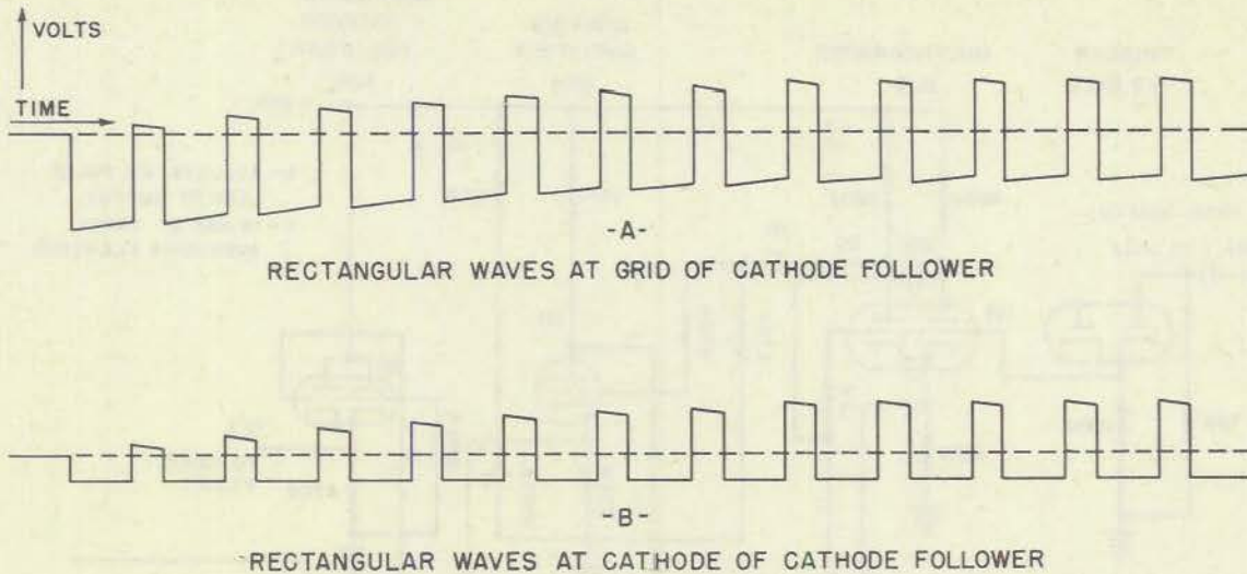
Fig. 10 - Transient response of averaging circuit
