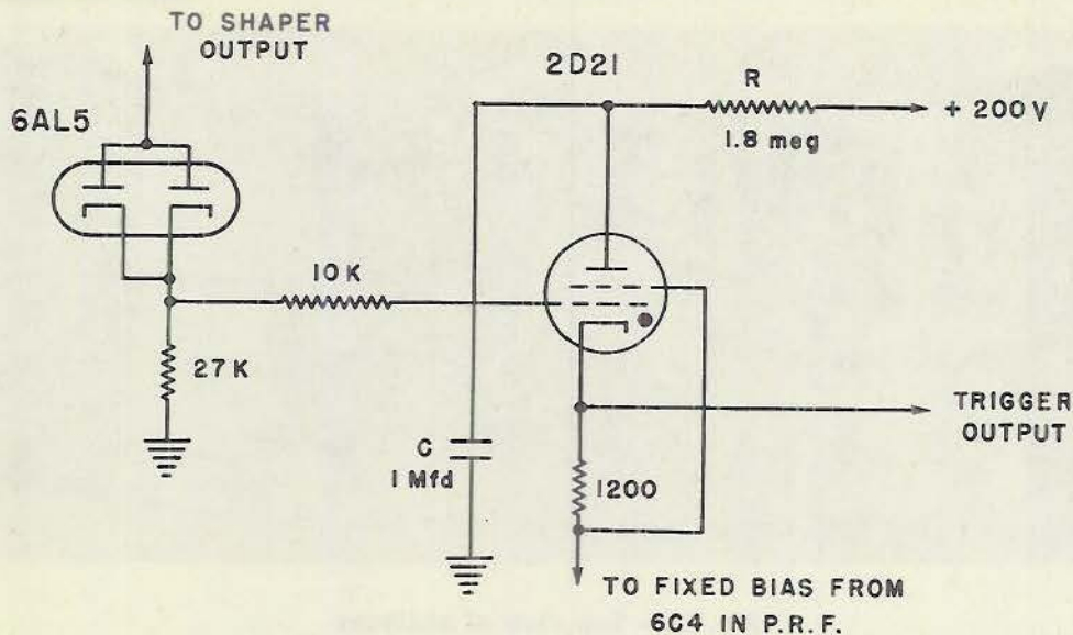
Fig. 14 - Automatic reset trigger circuit
