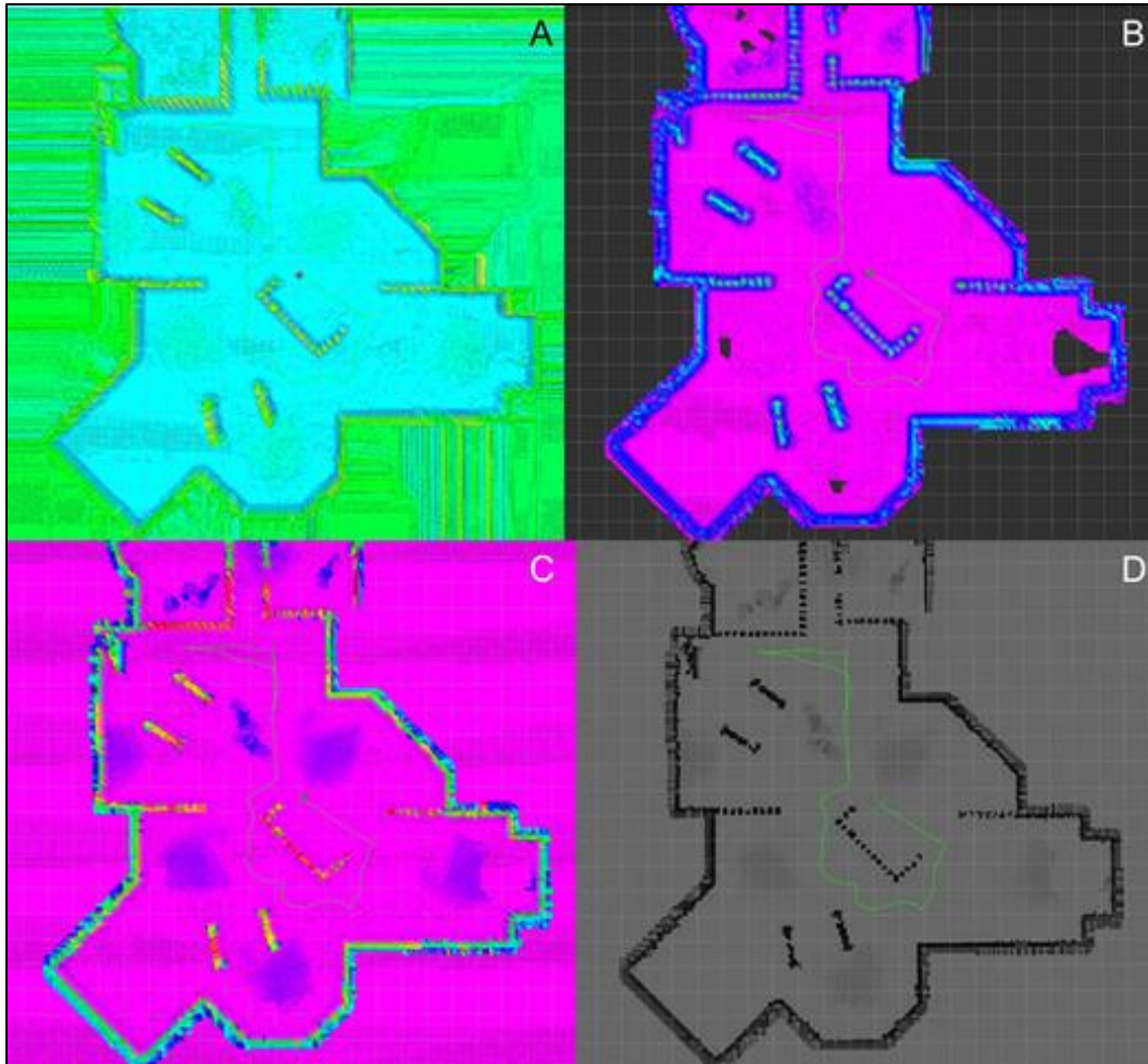
Figure 12. Traversability grid map and 2.5D occupancy grid of the Office Construction World. A , B , and C , respectively, show the edges, roughness, and traversability. D shows the occupancy grid.
