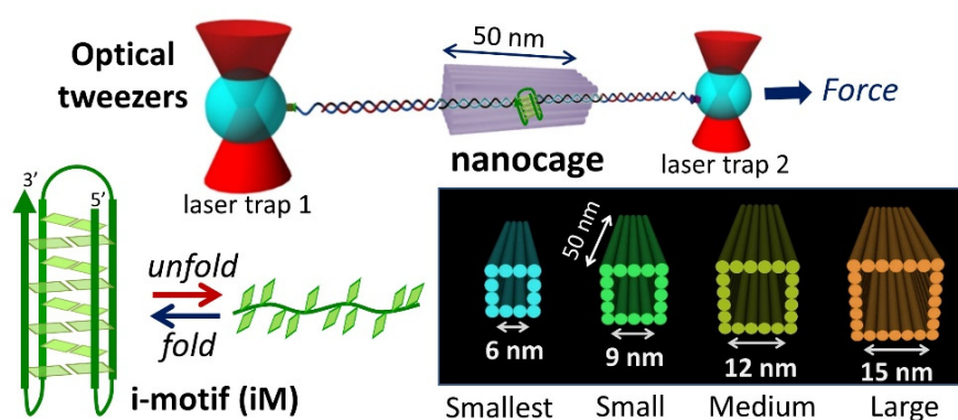
Fig. 1 Schematic illustration of i-motif in the DNA nanocage and the method to unfold/fold i-motif structure inside the four different size of nanocages using optical tweezers.
