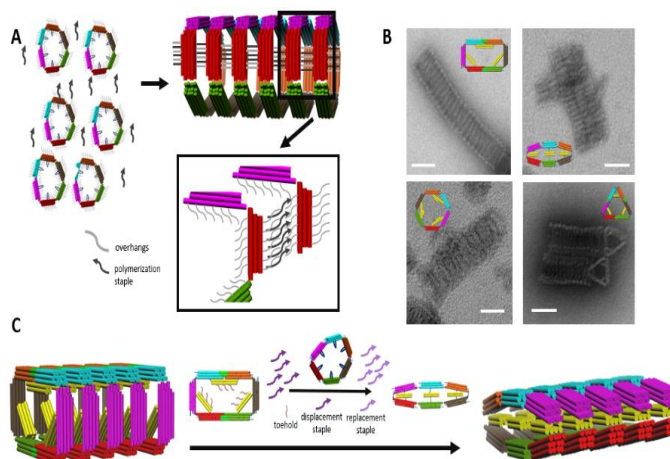
Figure 2: Polymerization and Reconfiguration of tubes. A depicts the polymerization schematic of the 6-bar using 8bp and 12bp overhangs on each bundle. Polymerization strands are added to bind the monomer structures together. B TEM images of polymerized 6-bar structures. Top left rectangle, top right compact configuration, bottom left hexagon, bottom right triangle. Scale bars = 50nm C Schematic depicting a rectangle reconfiguring to compact configuration. Toeholds are placed on the truss staples, then strand displacement occurs to form an intermediate state. Replacement staples are then used to reconfigure the polymer to a compacted configuration.
