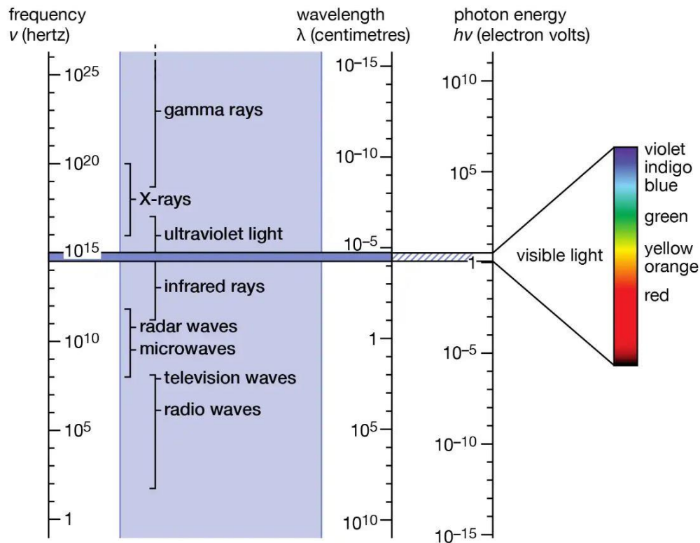
Figure 3. The electromagnetic spectrum (Encyclopædia Britannica, 2023).
