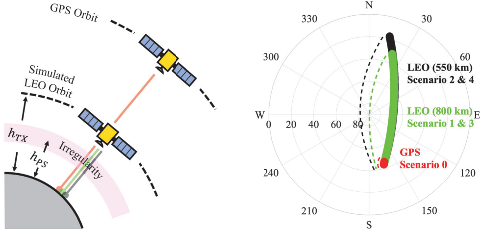
Figure 3: (a) Scintillation simulation configuration. (b) Sky plot of GPS satellite and LEO satellites at 550 and 800km altitude during the 500-second interval
