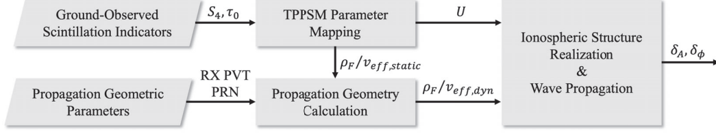
Figure 2: Flow chart of the ionosphere scintillation simulator presented in Xu et al. (2020)
