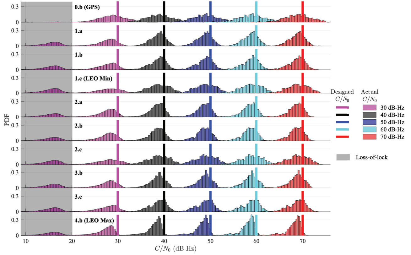
Figure 7: Distributions of receiver estimated C/N_0 dependence on set C/N_0
