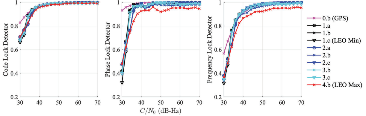
Figure 6: Average DLL, PLL, and FLL lock detector values for each simulation scenario and C/N_0 values
