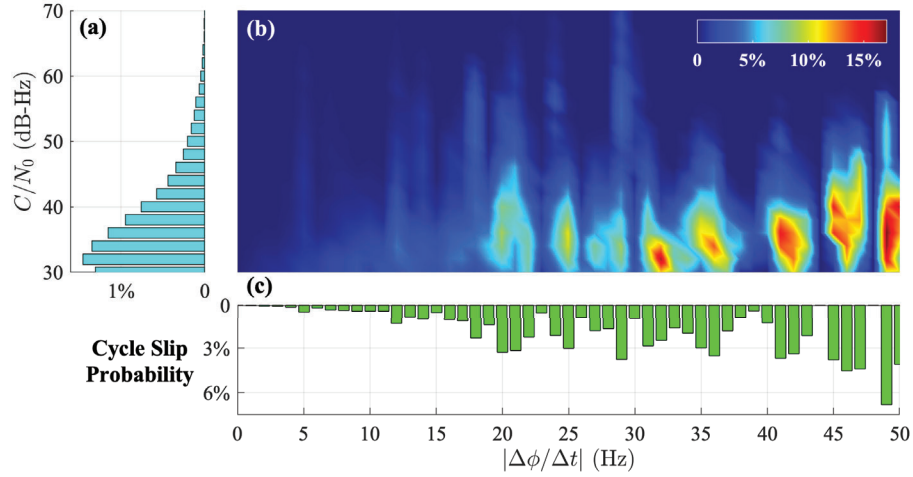
Figure 9: Cycle slip probability at different phase rate disturbance and C/N_0 values
