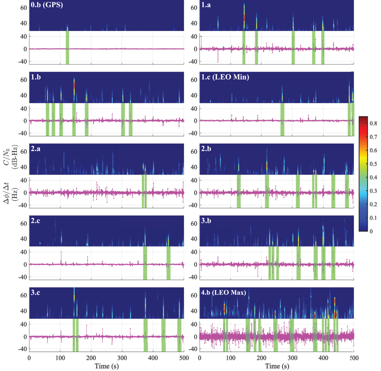
Figure 12: Cycle slip probability at different times and C/N_0 (top) calculated from repeat simulations and corresponding phase rate disturbance (bottom)
