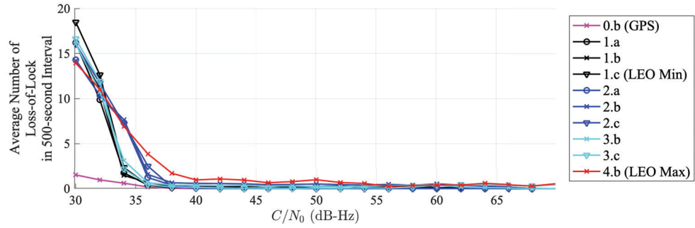
Figure 10: Average number of loss-of-lock during the 500-s interval as function of C/N_0 for each simulation scenario
