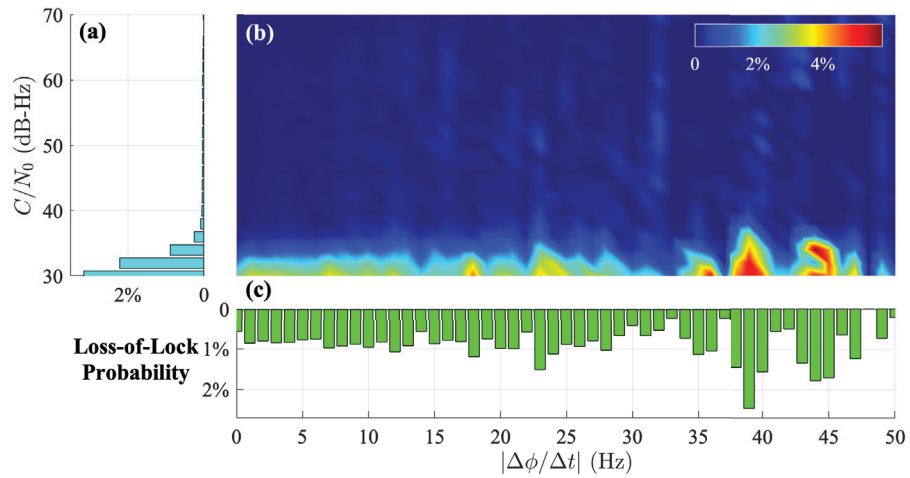
Figure 11: Loss-of-lock probability at different phase rate disturbance and C/N_0
