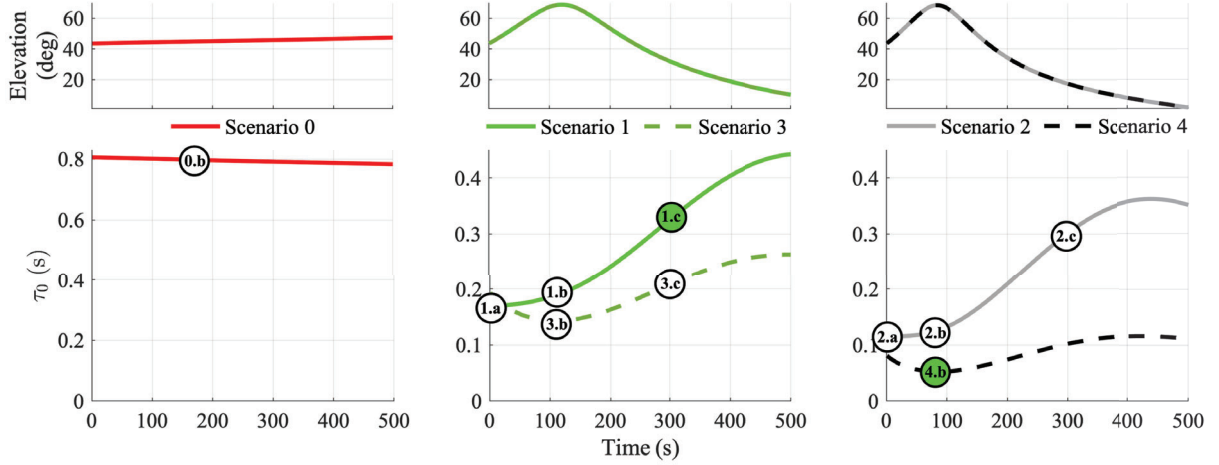
Figure 4: Satellite elevation (top), and decorrelation time \tau_0 (bottom) of 5 scenarios duration the 500-second interval
