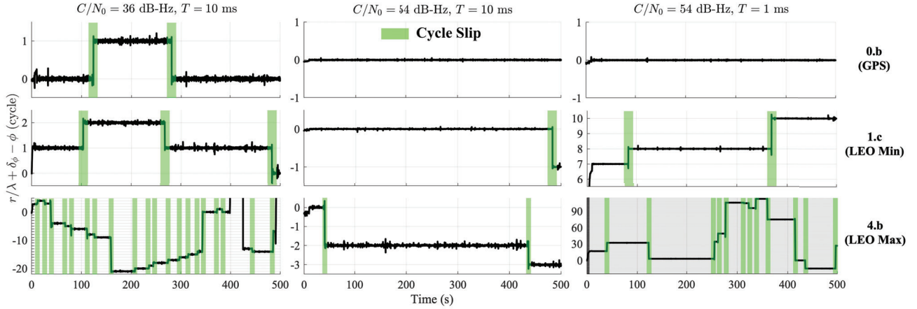
Figure 8: Carrier phase tracking error in sub-scenario 0.b (GPS), 1.c (LEO min), and 4.b (LEO max) at C/N_0 of 36 and 54 dB-Hz
