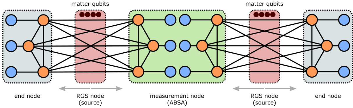
Figure 2: Network link
