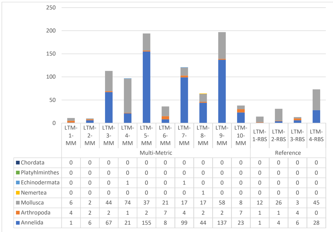
Figure 3-2. Faunal Composition
