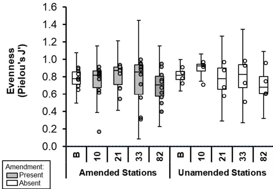
Figure 11: Evenness.
