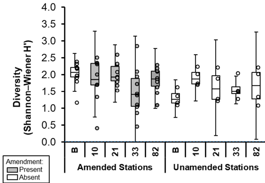
Figure 10: Diversity.
