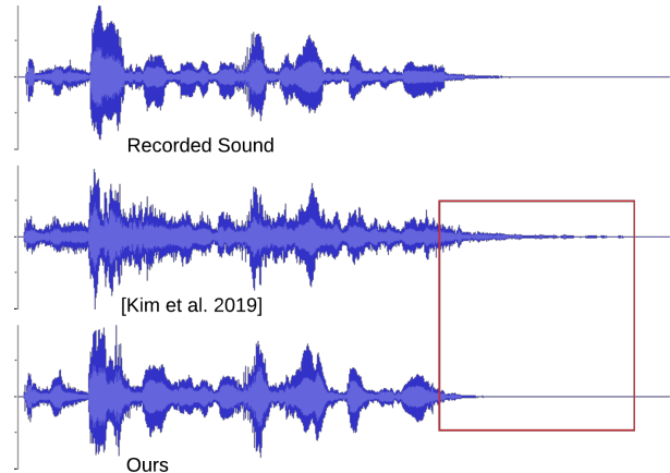
Fig. 11: We demonstrate the importance on T_{60} optimization on the audio amplitude waveform. Our method optimizes the material parameters based on input audio and matches the tail shape and decay amplitude with the recorded sound, whereas the visual-based object materials from Kim et al. [29] failed to compensate for the audio effects.
